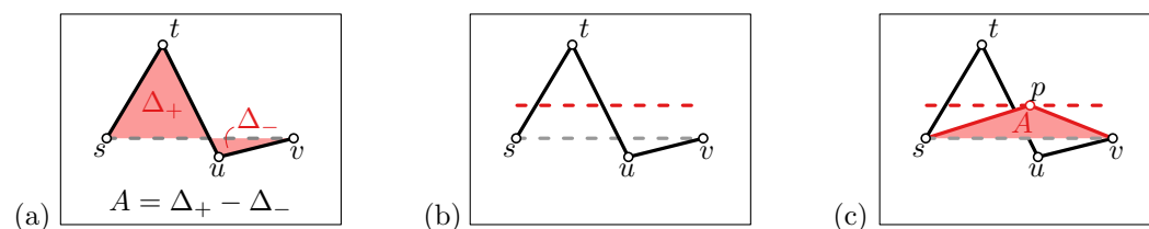
■ Figure 5 (a) Area contributed by the original rung and its adjacent edges. (b) The area-equivalence line. (c) Any position of the area-equivalence line creates a triangle that contributes the same area as before. (Suboptimal position selected for visualization purposes.)
