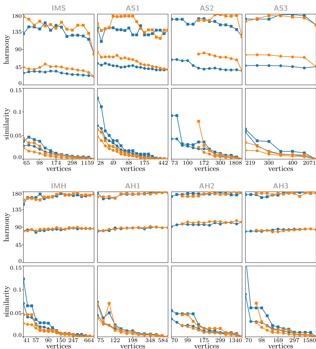
■ Figure 14 Average (circles) and maximum (squares) harmony and similarity as the algorithms simplify the input; lower values are better. Blue: harmonious algorithm; orange: isolated algorithm. Note that the horizontal axis is not linear. The maximum similarity (0.27) for the result of our harmonious algorithm on AH3 with 81 vertices has been cropped.
