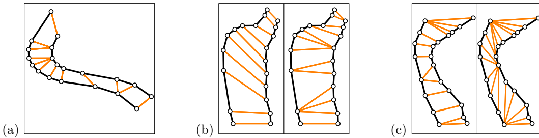
■ Figure 2 (a) The polyline matching should be monotone. (b) The DTW matching (left) minimizes the number of matched pairs instead of preserving locality (right). (c) Matchings with the same Fréchet distance; the left matching is locally correct.
