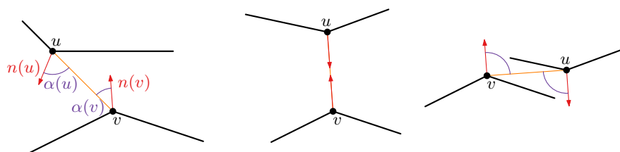
■ Figure 12 (left) The harmony measure for a matched pair (u, v) is the sum of the angles indicated in purple (\alpha(u) + \alpha(v)) . Note that the direction of the normal is irrelevant for the score. (middle) A “perfect” pair, scoring zero. (right) A “worst” pair, scoring 180 degrees.
