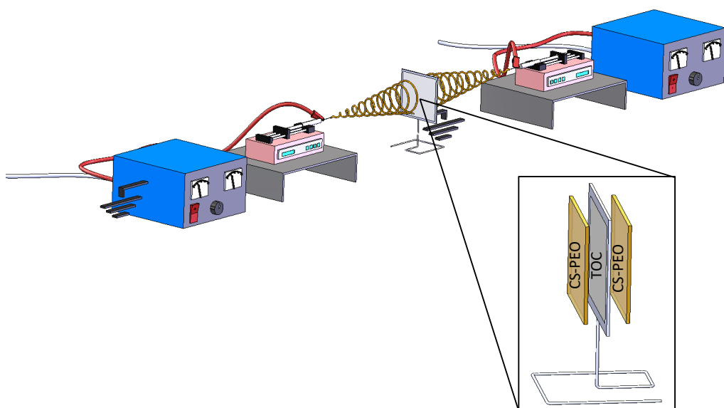
Fig. 1 Experimental set-up of electrospinning for the preparation of the CS-PEO/TOC bio-based composite
