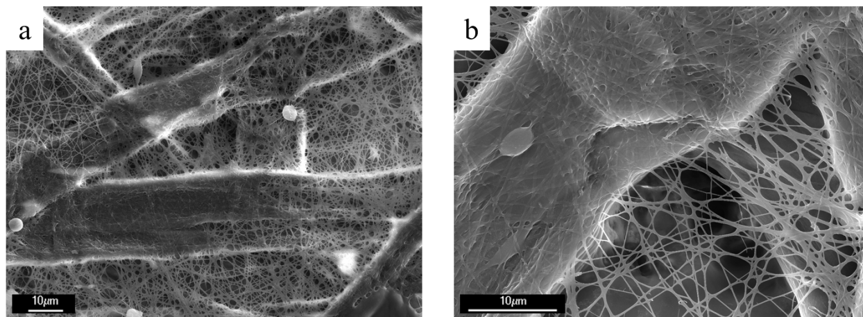
Fig. 5 Morphology of the 3CS-PEO/TOC bio-based composite after neutralization treatment with \text{NaHCO}_3 at (a) x 1500 and (b) x 2500 magnifications
