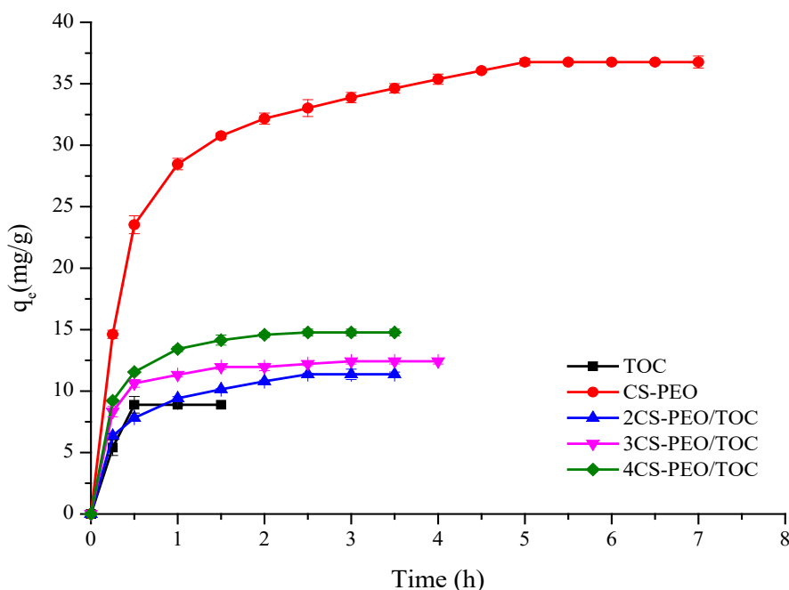
Fig. 8 Effect of contact time on the adsorption of copper ions onto the five different biocomposites
