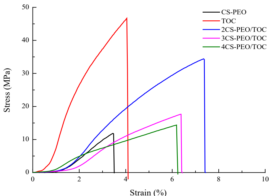
Fig. 7 Stress-Strain curves for CS-PEO, TOC and xCS-PEO/TOC
