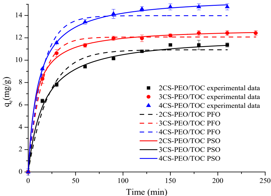
Fig. 9 Pseudo-first order and Pseudo-second order model of copper ions adsorption onto the xCS-PEO/TOC biocomposite
