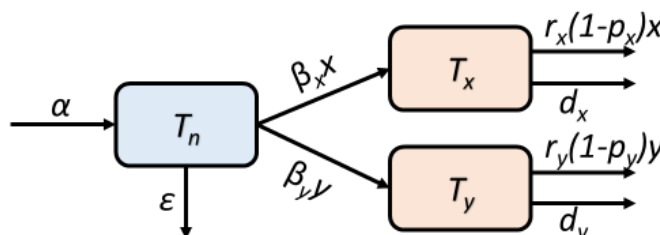
Figure 2. The T-cell regulatory pathway, which involves the naïve T-cells, is denoted T_n . The baseline production rate is denoted \alpha and natural elimination rate \epsilon . The pathogen specific cytotoxic T-cells are produced from this T-cell regulatory pathway. The amount of cancer cells is denoted by x , while that of infected cells is denoted by y . The amount of the cancer specific effector cells is denoted T_x and is produced with the per capita rate \beta_x x while the amount of the infection specific effector cells is denoted T_y and is produced with the per capita rate \beta_y y . The effector cells have natural death rates d_x and d_y , respectively. In addition, active cytotoxic T-cells may become inactivated or exhausted, which adds an extra removal from the pools of active cytotoxic T-cells. The removal per time is assumed proportional to the respective binding with cancer cells and infected cells multiplied by the probabilities 1 - p_x and 1 - p_y , respectively.
