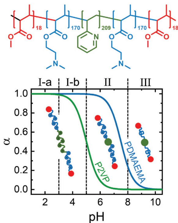
Figure 1. Chemical structure of the non-charged pentablock terpolymer and calculated degrees of ionization, \alpha , of P2VP (green line, pK_{a,P2VP} \cong 5.0 ) and PDMAEMA (blue line, pK_{a,PDMAEMA} \cong 7.5 ) as a function of pH, using \alpha = (1 + 10^{pH-pK_a})^{-1} . [47] The red circles denote the hydrophobic PMMA end blocks. The regimes based on the different charge states of the pentablock terpolymer are indicated: I-a) P2VP and PDMAEMA are fully charged and hydrophilic. I-b) PDMAEMA is fully charged and P2VP is partially charged. II) P2VP is weakly charged or uncharged and hydrophobic, PDMAEMA is still highly charged and hydrophilic. III) P2VP is uncharged and hydrophobic, PDMAEMA is weakly charged or uncharged and remains hydrophilic.
