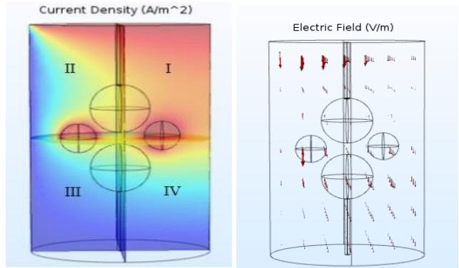
(b) Fig. 4 - Pattern of electric field and current density of SF 6 for (a) Normal condition; (b) Presence of pressure
