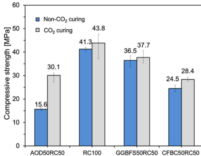
Fig. 2 - Compressive strength of all four \text{CO}_2 sequestered materials at 14 th day [2]
