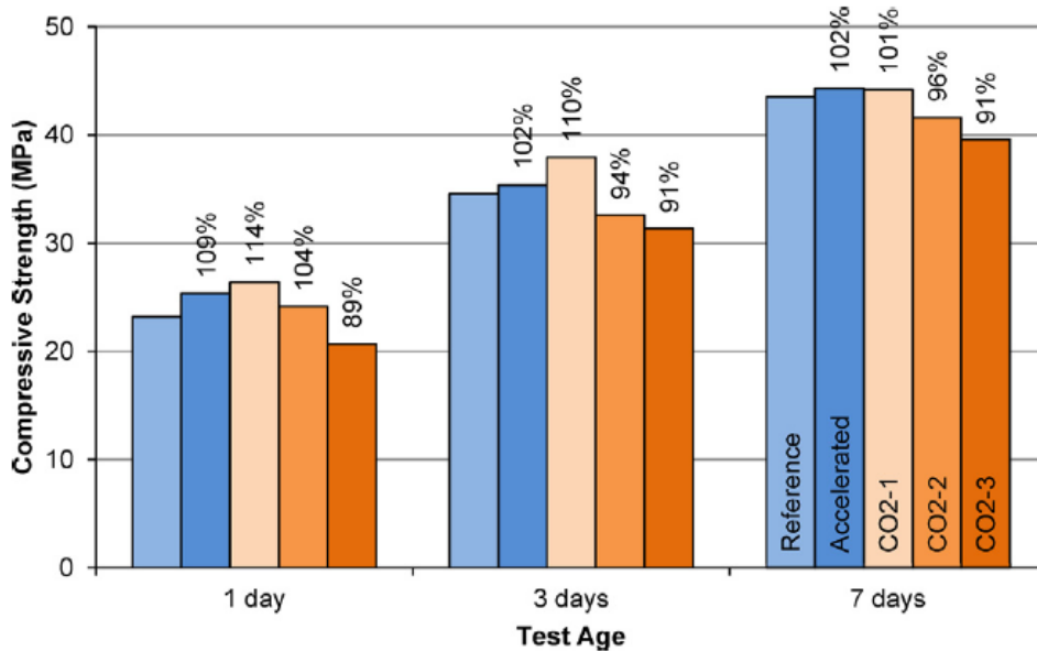
Fig. 5 - Early age compressive strength of concrete [13]
