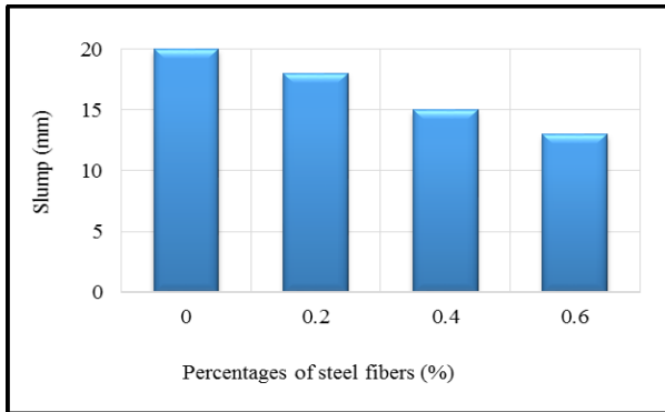
Fig. 4 The slump values of POBC-concrete with steel fibers
