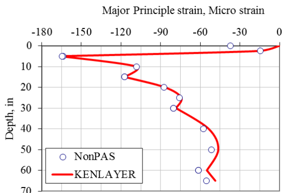
Fig. 7 Major principle strain vs. Depth.
