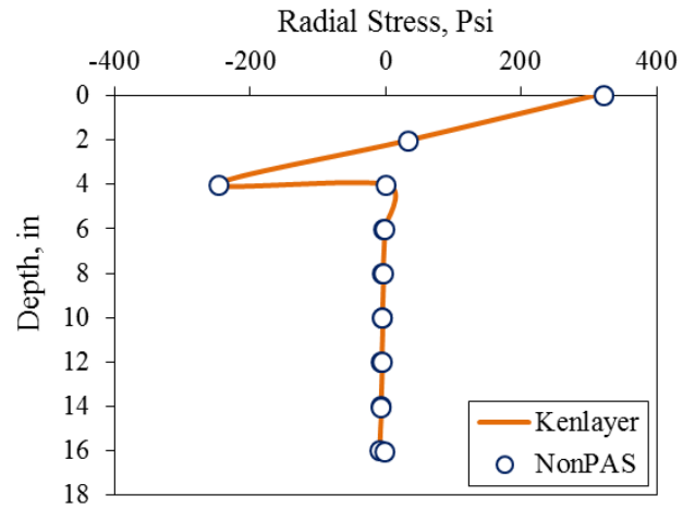
Fig. 12 Radial stress vs. depth (SLD=0.0).
