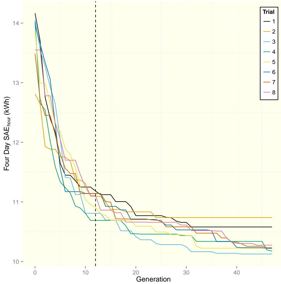
Figure 5: The plot shows the convergence of the best individual in each trial of Experiment 4 when the abbreviated schedule is used (i.e., the first 75% of the evaluations). The dotted line marks generation 12, which is 25% of the 1,024 evaluations allotted to the abbreviated schedule. Before this point, individuals produced by the abbreviated schedule tuning are not particularly useful as seeds because of their relatively high SAE.
