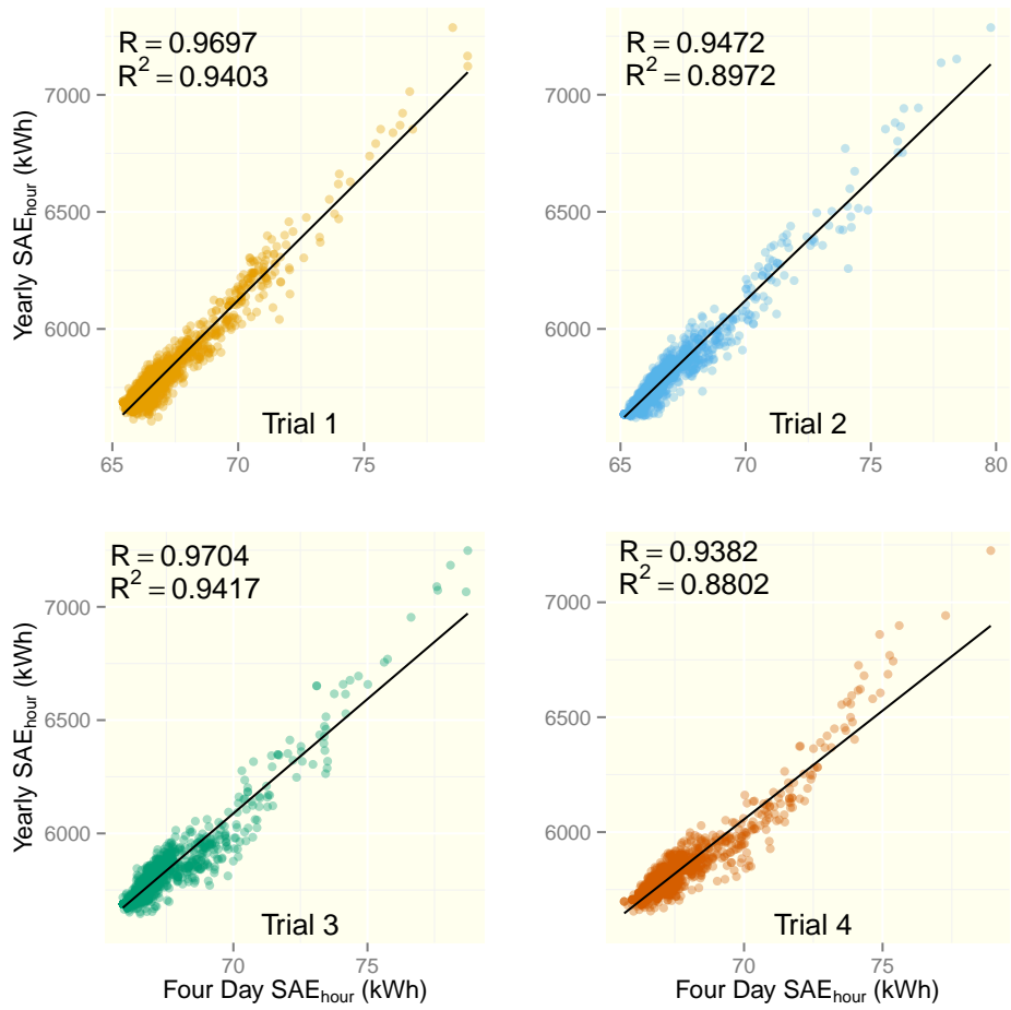
Figure 3: Each of the four independent trials shows a very high correlation between the 4 day and full-year-schedule SAE of hourly electrical usage. This means that an abbreviated surrogate (4 -day schedule) is a plausible method of expediting the tuning.
