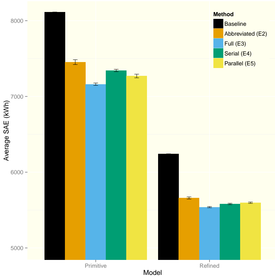
Figure 6: The graph shows the results of Experiments 2–5 compared with the baseline (see Table 6). The average minimum SAE value found across all eight trials represents each method, and each method is accompanied by standard error bars (except for the baseline). The y-axis minimum value was increased to 5,000 to highlight the differences between the methods.
