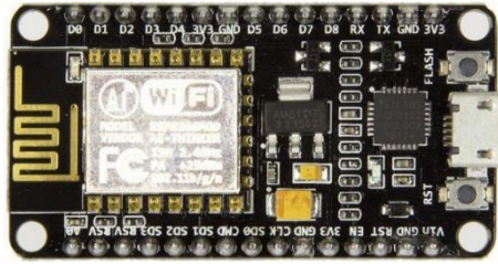
Figure 11. NodeMCU Development Board based on ESP8266
