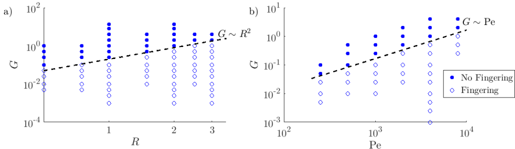
FIGURE 10. Stable vs. unstable displacements for (a) Pe = 4000 and (b) R = 2 . Filled circles denote simulations where no fingers were observed during the entire length of the simulations, while unfilled circles denote simulations where fingers were observed for at least some portion of the simulation. Dashed lines show the stability boundary G = 5 \times 10^{-5} R^2 Pe .
