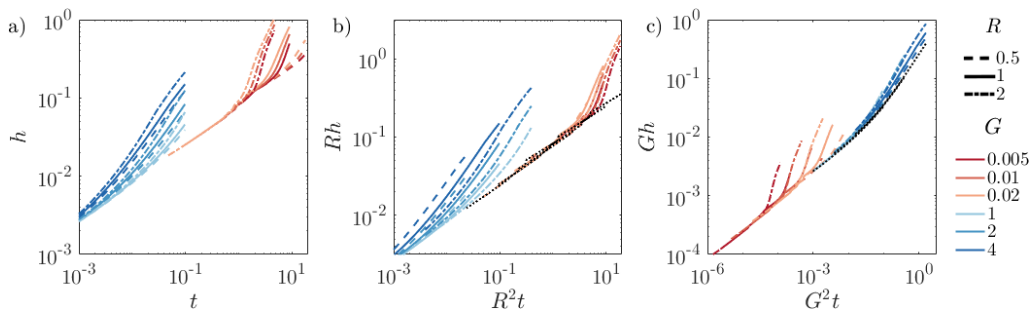
FIGURE 6. Plots of h(t) for Pe = 100 and different G and R as labelled. The raw data is plotted in (a). In (b) the spreading length is rescaled by the predicted scalings for the small- G slumping limit. The dotted lines denote simulations with G = 0 and R = \{0.5, 1, 2\} . In (c) the spreading length is rescaled by the predicted scalings for the large- G slumping limit. The dotted lines denote simulations with R = 0 and G = \{1, 2, 4\} .
