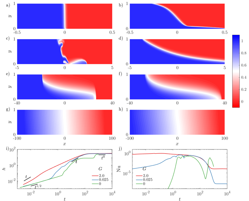
FIGURE 4. Colourmaps of the concentration field for (R, Pe) = (2, 500) and (a,c,e,g) G = 0.025 , (b,d,f,h) G = 2 . The snapshots are taken at times (a,b) t = 0.05 , (c,d) t = 2 , (e,f) t = 30 , and (g,h) t = 500 . Evolution of (i) the spreading length, h and (j) the Nusselt number, Nu , for the same parameters as (a-h).
