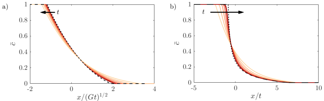
FIGURE 7. Evolution of the transversely averaged concentration (or equivalently the height of the current above the base) found by solving (4.7) for (a) small-times, (R, G) = (2, 8) and t ranging logarithmically from 0.03 to 1 and (b) large-times, (R, G) = (2, 2) and t ranging logarithmically from 1 to 32. The small-time asymptotic limit found by solving (4.8) and large-time asymptotic limit (4.10) are given by dashed black lines.
