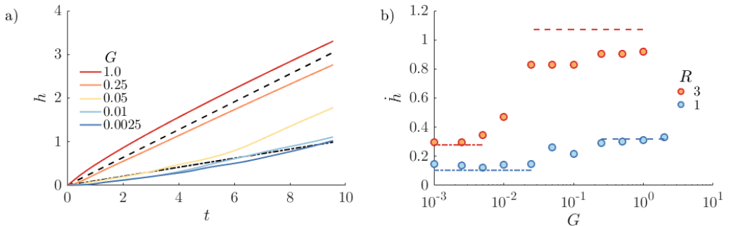
FIGURE 9. Plot of h(t) for (R, Pe) = (1, 4000) and different values of G in the intermediate-time regime. (b) Plot of the spreading rate \dot{h} calculated by least-squares fitting a function of the form h = h_0 + \dot{h}t to the numerical results for t in the range 5 \leq t \leq 10 , for Pe = 4000 and different G and R . The theoretical predictions for h in (a) and \dot{h} in (b) are found from the solution (4.10) with either M = e^R or M = e^R \text{erf}(\sqrt{R}) / \text{erfi}(\sqrt{R}) , given by dashed and dot-dashed lines respectively.
