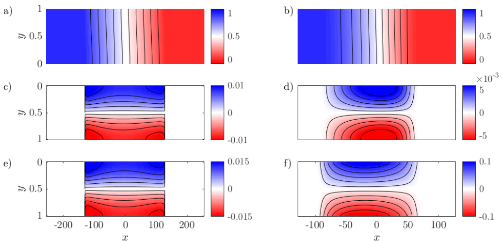
FIGURE 11. Colourmaps (with overlain contours) of the (a,b) concentration field, (c,d) concentration deviations c' , and (e,f) streamwise velocity, u for (a,c,e) (R, Pe, G, t) = (1.5, 1000, 0.1, 1000) (small G ) and (b,d,f) (R, Pe, G, t) = (1.5, 100, 10, 1000) (large G ). The left panels correspond to flow in the shutdown regime and the right panels correspond to flow in the viscously-enhanced Taylor slumping regime. Note that the aspect ratio of the figures is compressed, so variations in the x -direction seem more pronounced than they actually are.
