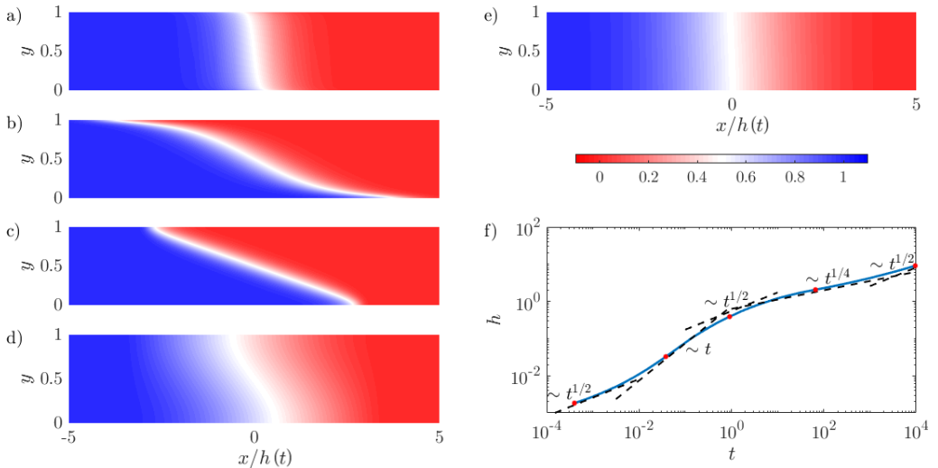
FIGURE 2. Evolution of the concentration field for R = 0 and (G, Pe) = (3, 100) . (a-e) Plots of the concentration field vs. x/h(t) and y at (a) t = 1 \times 10^{-4} , (b) t = 0.036 , (c) t = 0.83 , (d) t = 57 (e) t = 8000 . (f) Evolution of the spreading length, h , as a function of time, t . The dots correspond to the snapshots (a-e) and the dashed lines correspond to the theoretical predictions from Szulczewski & Juanes (2013).
