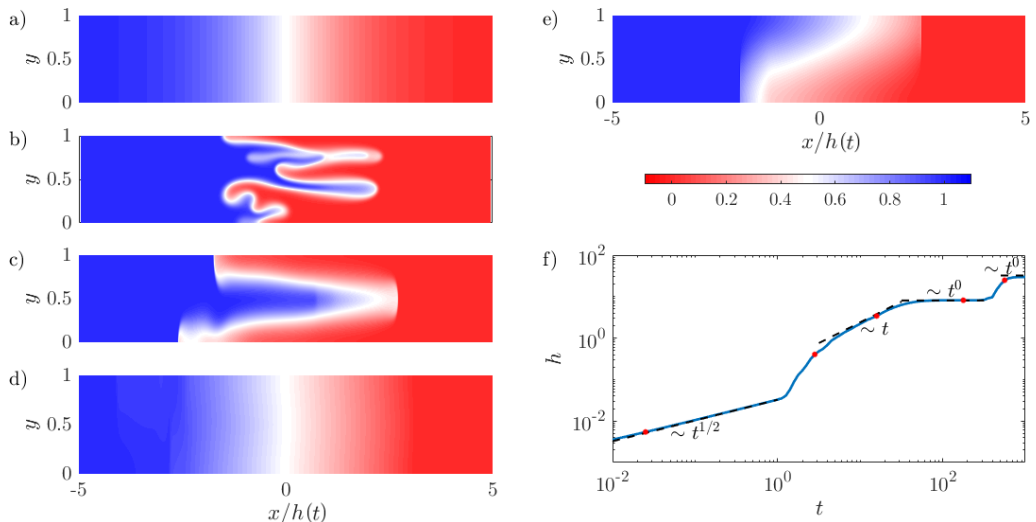
FIGURE 3. Evolution of the concentration field for G = 0 and (R, \text{Pe}) = (2.5, 500) . (a-e) Plots of the concentration field vs. x/h(t) and y at (a) t = 2 \times 10^{-2} , (b) t = 2.6 , (c) t = 15 , (d) t = 170 (e) t = 525 . (f) Evolution of the spreading length, h , as a function of time, t . The dots correspond to the snapshots (a-e) and the dashed lines correspond to the theoretical predictions from Nijjer et al. (2018).
