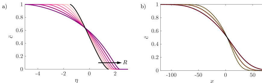
FIGURE 13. (a) The similarity solution of (4.25) for R = 0, 0.5, 1, 1.5, 2, 2.5, 3 . The analytical solution for R = 0 is given by the black line (Szulcowski & Juanes 2013). (b) The evolution of \bar{c} for (R, \text{Pe}, G) = (3, 10, 10) at t = \{1000, 2000, 4000\} . The theoretical predictions, found by solving (4.24), are denoted by dotted lines.
