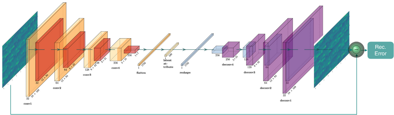
Fig. 2. The convolutional auto-encoder (CAE) architecture with 4 encoder layers and 4 decoder layers as an example. An encoder layer is a sequence of convolution – batch-normalisation – PReLU – max-pooling . A decoder layer is a sequence of transposed convolution – batch-normalisation – PReLU – transposed max-pooling . The distance between the original and reconstructed image represents the reconstruction error.
