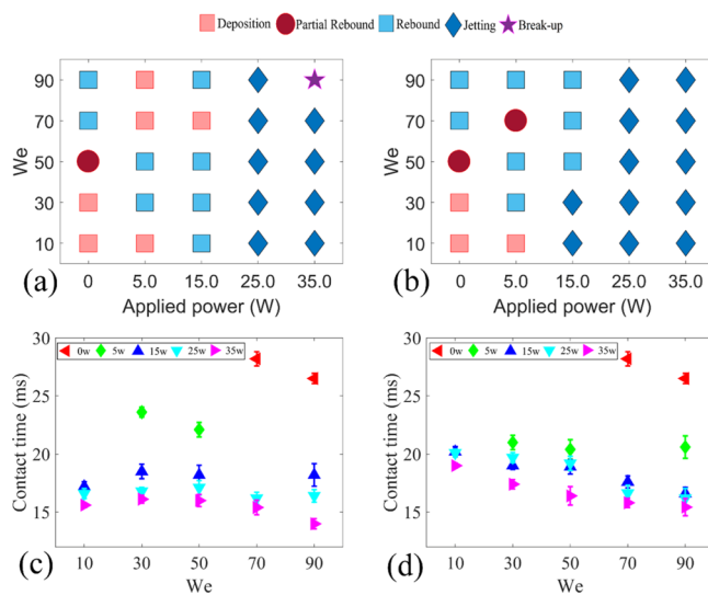
Figure 8. Droplet impact regime maps as functions of applied SAW power and We number for (a) USAW and (b) DSAW cases. Contact time vs We number for different applied SAW powers for (c) USAW and (d) DSAW scenarios. In all the experiments, a droplet with a volume of 3.5 \mu\text{L} has an impact on a ZnO/Si SAW device with an inclination angle of 15^\circ .
