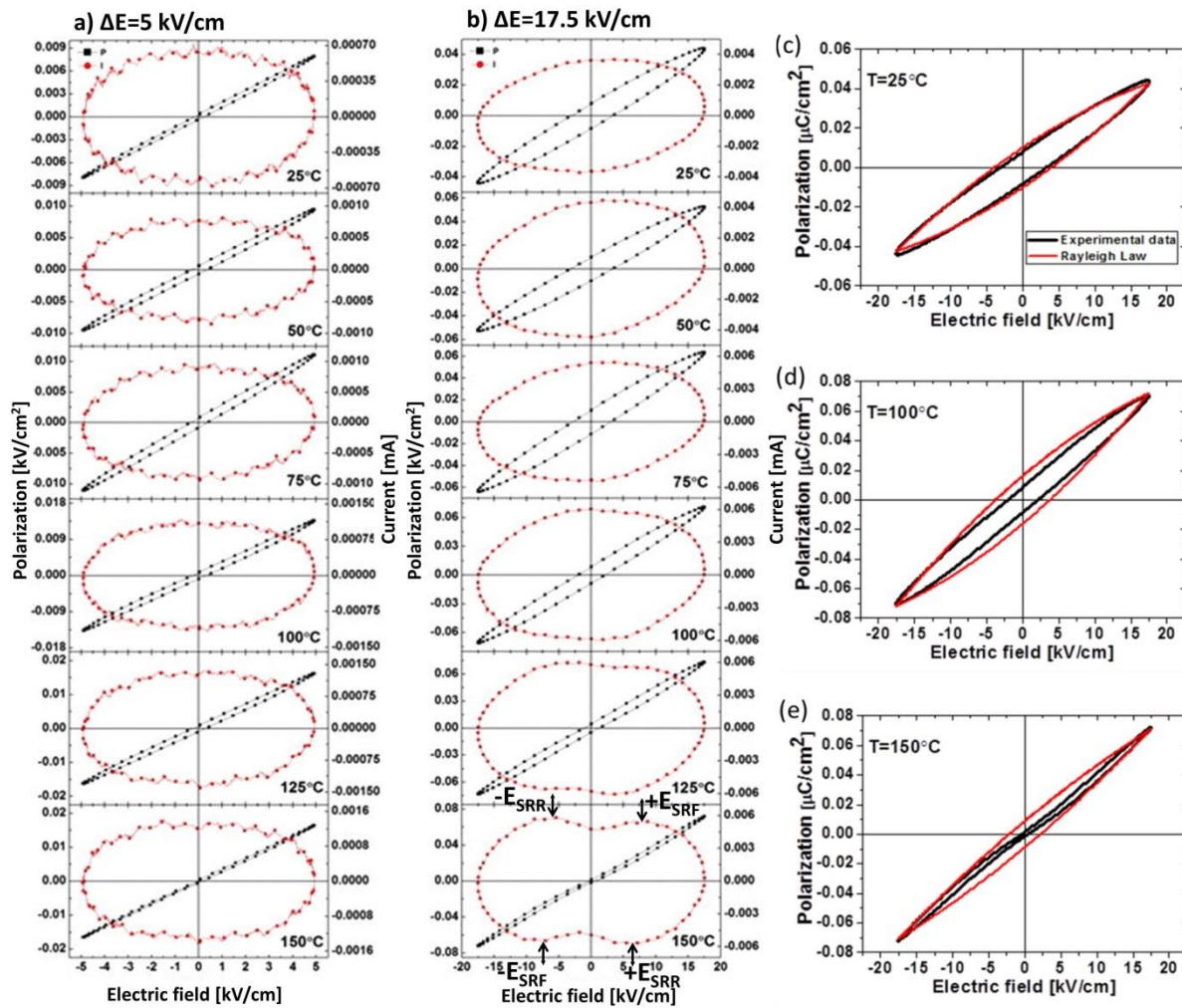
Figure 25. Rayleigh-like loops of 0.95[0.94(\text{Bi}_{0.5}\text{Na}_{0.45}\text{Li}_{0.05})\text{TiO}_3-0.06\text{BaTiO}_3]-0.05\text{CaTiO}_3 ceramics in the temperature range 25^\circ\text{C} - 150^\circ\text{C} at 5 Hz frequency: (a) current-polarization-electric field loops at 5 kV/cm electric field amplitude; and (b) current-polarization-electric field loops at 17.5 kV/cm electric field amplitude [Reproduced from Ref.238
