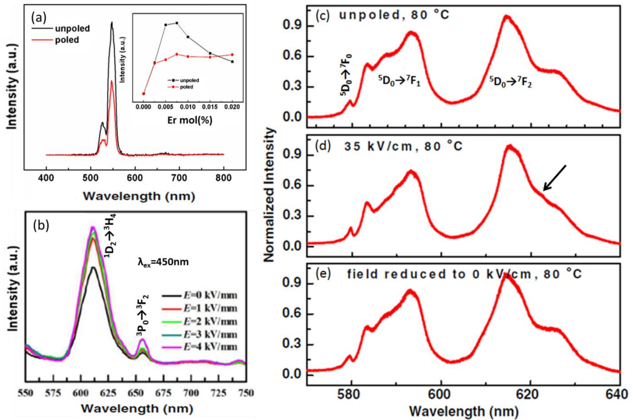
Figure 39. Effects of an applied electric field on the photoluminescence properties of (a) Er-doped 0.94\text{Bi}_{0.5}\text{Na}_{0.5}\text{TiO}_3\text{-}0.06\text{BaTiO}_3 at room temperature [Reproduced with permission from Ref.321 Copyright 2015 John Wiley and Sons]; and (b) Pr-doped 0.93\text{Bi}_{0.5}\text{Na}_{0.5}\text{TiO}_3\text{-}0.07\text{BaTiO}_3 at room temperature [Reproduced with permission from Ref.159 Copyright 2015 American Chemical Society]. Variations of the photoluminescence spectrum of 0.94(\text{Bi}_{0.5}\text{Na}_{0.5})\text{TiO}_3\text{-}0.06\text{BaTiO}_3 at 80^\circ\text{C} in as-sintered state (c), under an electric field of 35\text{ kV/cm} (d) and after removing the electric field (e) [Reproduced with permission from Ref.320 https://journals.aps.org/prl/abstract/10.1103/PhysRevLett.116.117601
