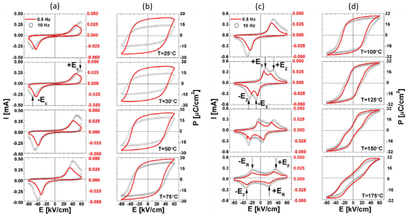
Figure 12. Temperature and frequency dependence of I-P-E loops in the range 25°C-75°C (a)-(b) and 100°C-175°C (c)-(d) for 0.95[0.94(\text{Bi}_{0.5}\text{Na}_{0.5})\text{TiO}_3-0.06\text{BaTiO}_3]-0.05\text{CaTiO}_3 .
