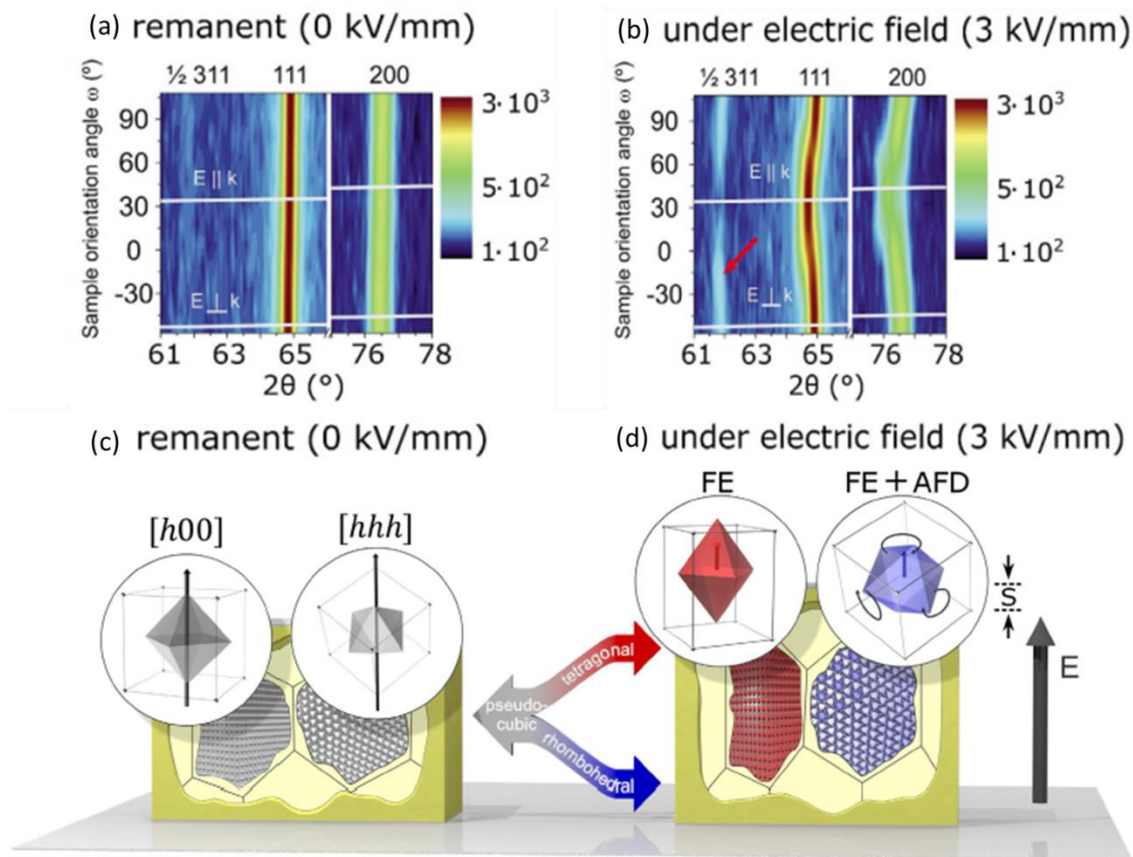
Figure 31. (a)-(b) Diffraction patterns at different sample's orientation angles in the range -57^\circ \leq \omega \leq 108^\circ of remanent state at 0 kV/mm after applying an electric field of 30 kV/cm (a) and under an applied electric field of 30 kV/cm (b). The 2\theta ranges selected include \frac{1}{2} 311 , 111 and 200 reflections. The white lines trace the patterns obtained in the conditions of k \parallel E and k \perp E . The red arrow in figure (b) indicates the maximum intensity of the \frac{1}{2} 311 reflection. (c) Scheme of grains with [h00] and [hhh] in the pseudo-cubic structure in the remnant state. (d) Structural transformation of pseudo-cubic grains to tetragonal (red) and rhombohedral (blue) symmetry due to ferrodistortive and ferrodistortive+antiferrodistortive instabilities, respectively. [Reproduced with permission from Ref.257]
