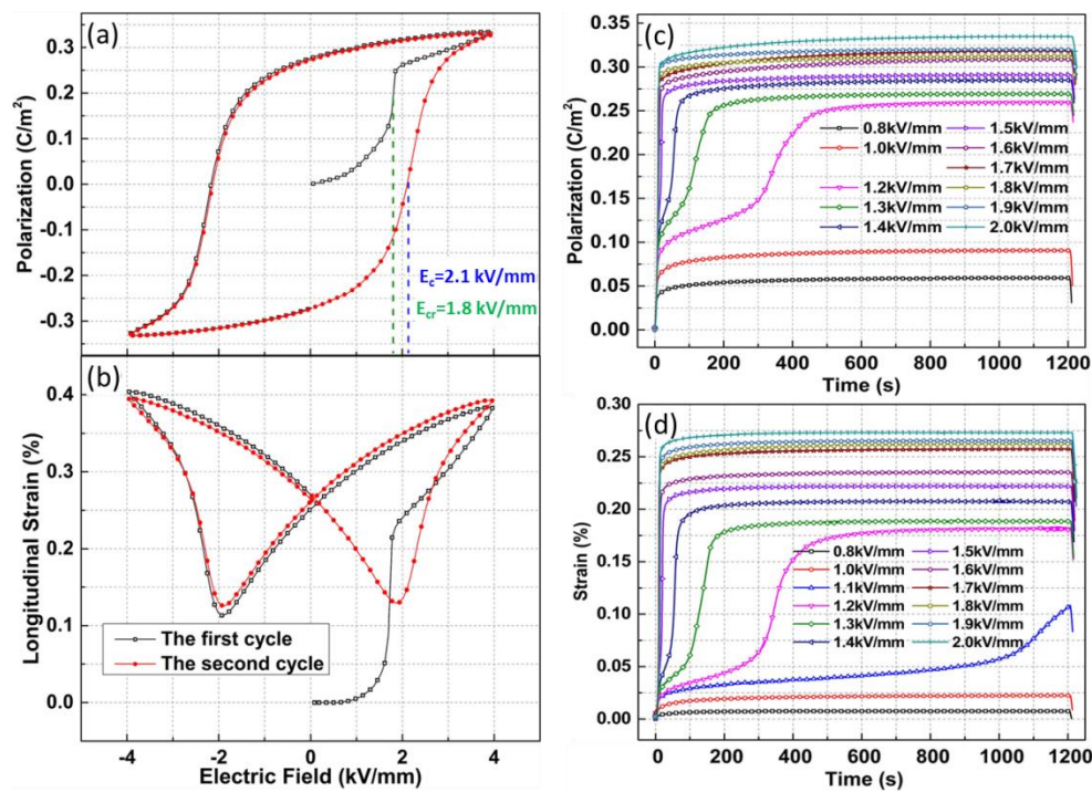
Figure 26. Hysteresis loops and creep curves of 0.93BNT-0.07BT: (a) polarization-electric field loop; (b) strain-electric field loop; (c) polarization creep curves; and (d) strain creep curves. [Reproduced from Ref.249 https://aip.scitation.org/doi/10.1063/1.4978704 with the permission of AIP Publishing].
