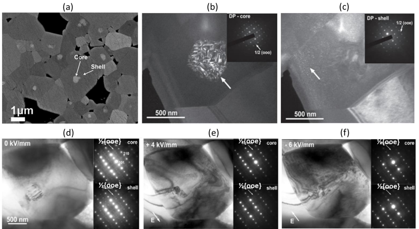
Figure 28. Microstructure of 0.75BNT-0.25ST ceramics. (a) SEM image of the core-shell structure in backscattering mode; (b)-(d) TEM images and local diffraction patterns of core and shell regions along the [112]_{pc} zone axis (b, c) and [120]_{pc} zone axis (d) under no applied field; (e), (f) TEM images and local diffraction patterns of core and shell regions under 40 kV/cm and -60 kV/cm, applied along the [001] direction. Superlattice reflections of the type \frac{1}{2}\{000\} and \frac{1}{2}\{00e\} are found in both core and shell. [Reproduced with permission from Ref.253 Copyright 2015 John Wiley and Sons].
