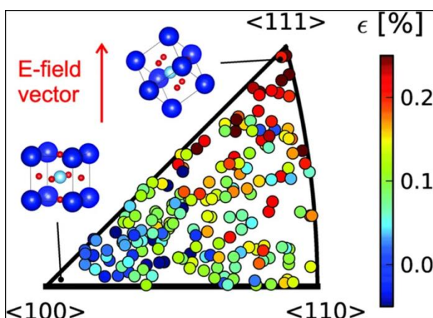
Figure 27. Strain map in grains of 0.82BNT-0.18BKT ceramics with different orientations with respect to the applied field. Each circle represents a single grain; the position of the circle is
