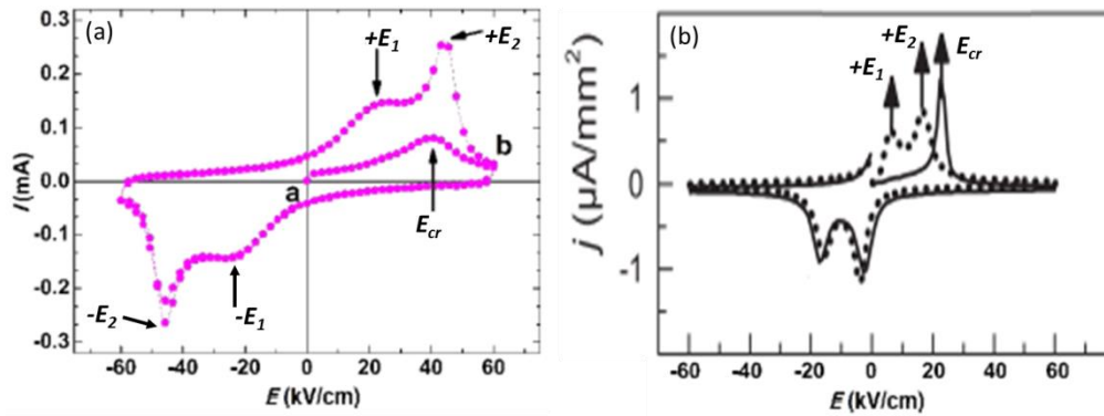
Figure 13. Current-electric field hysteresis loops from the very first cycle of (a) 0.95[0.94(\text{Bi}_{0.5}\text{Na}_{0.35}\text{Li}_{0.15})\text{TiO}_3-0.06\text{BaTiO}_3]-0.05\text{CaTiO}_3 [Reproduced with permission from Ref. 206 Copyright 2014 American Chemical Society] and (b) 0.97(\text{Bi}_{0.5}\text{Na}_{0.5})\text{TiO}_3-0.03\text{BaTiO}_3 doped with 0.5 mol% of Mn [Reproduced from Ref.207
