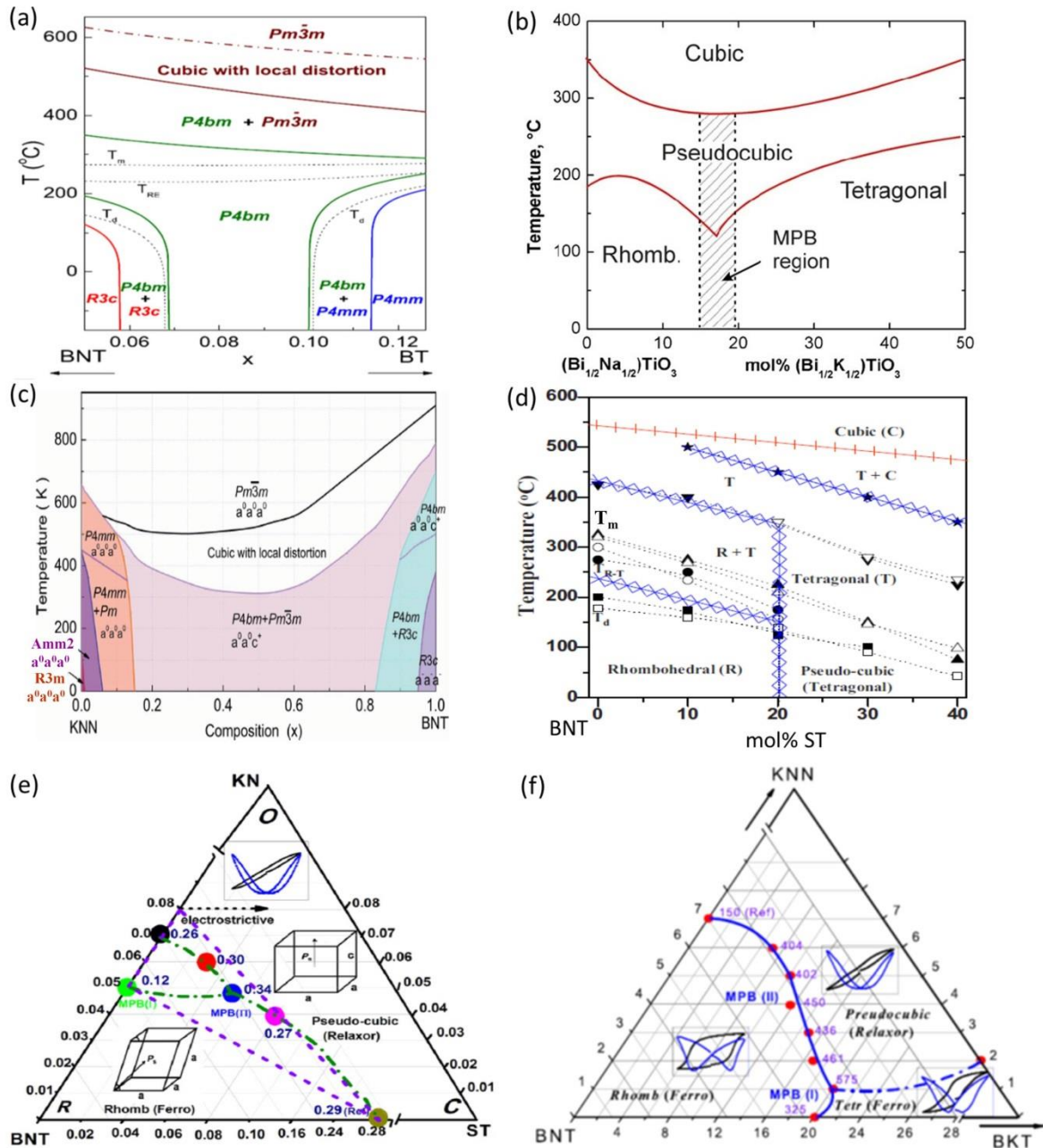
Figure 10. Phase diagrams of different BNT-based materials: (a) BNT-BT [Reproduced with permission from Ref.145 Copyright 2011 John Wiley and Sons]; (b) BNT-BKT [Reproduced with permission from Ref.146 https://iopscience.iop.org/article/10.1088/1468-6996/11/4/044302/meta with permission from Taylor & Francis]; (c) BNT-KNN [Reproduced with permission from Ref.147]; (d) BNT-ST [Reproduced from Ref.148 https://aip.scitation.org/doi/10.1063/1.3490781 with the permission of AIP Publishing]; (e) BNT-ST-KN [Reproduced with permission from Ref.150, Copyright 2015 Elsevier]; (f) BNT-BKT-KNN [Reproduced from Ref.151 https://aip.scitation.org/doi/10.1063/1.4795511 with the permission of AIP Publishing].
