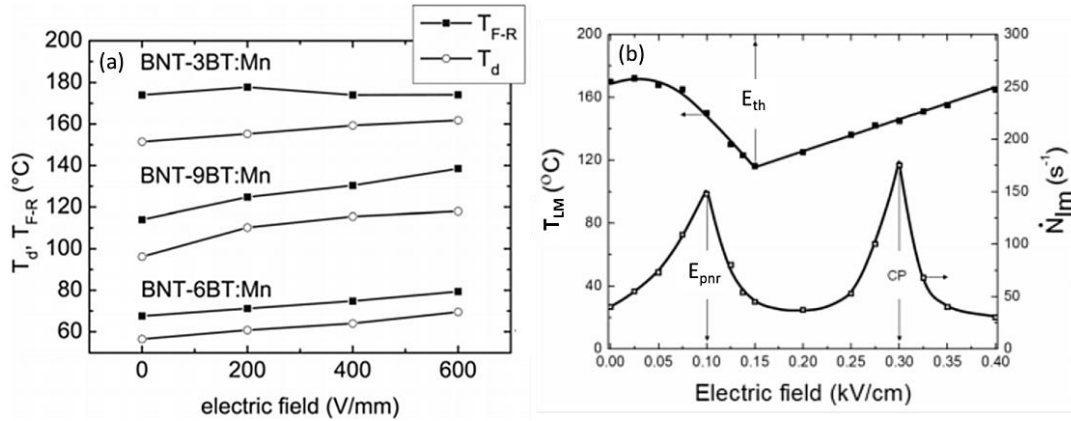
Figure 20. Dependence of characteristic temperatures on electric field bias: (a) T_d and T_{F-R} in (1-x)\text{Bi}_{0.5}\text{Na}_{0.5}(\text{Ti}_{0.995}\text{Mn}_{0.005})\text{O}_3-x\text{Ba}(\text{Ti}_{0.995}\text{Mn}_{0.005})\text{O}_3 [Reproduced from Ref.227 https://aip.scitation.org/doi/10.1063/1.3674275 with the permission of AIP Publishing]; and (b) T_{LM} and acoustic emission count rate in 0.94BNT-0.06BT [Reproduced from Ref.228 https://aip.scitation.org/doi/10.1063/1.5009326 with the permission of AIP Publishing].
