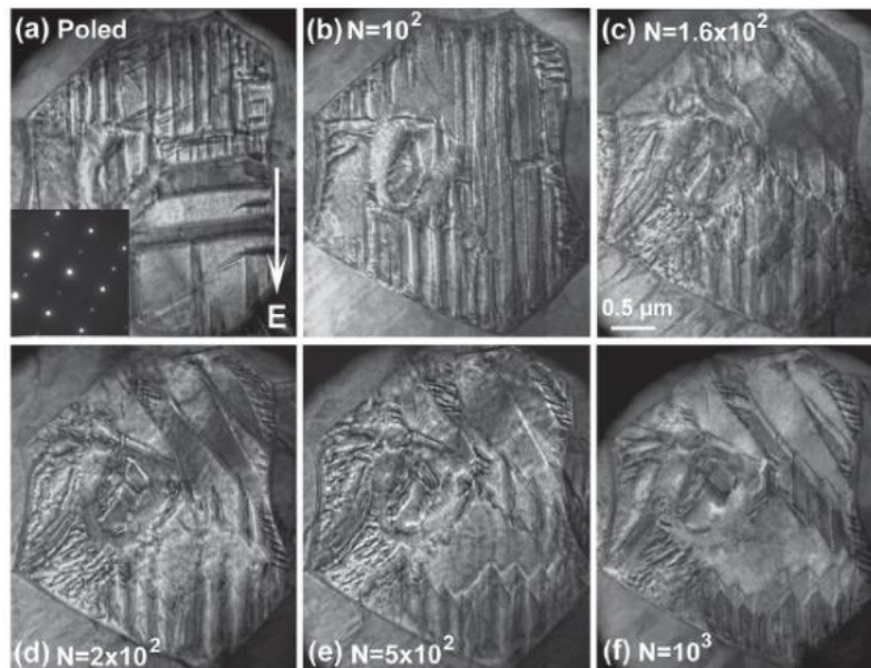
Figure 36: Evolution of the domains configuration during bipolar electrical cycles in [112]-aligned grain. The images are bright field micrographs taken: a) in the initially poled state at 30 kV/cm and after b) 100; c) 160; d) 200; e) 500; and f) 1000 cycles of bipolar electric fields.
