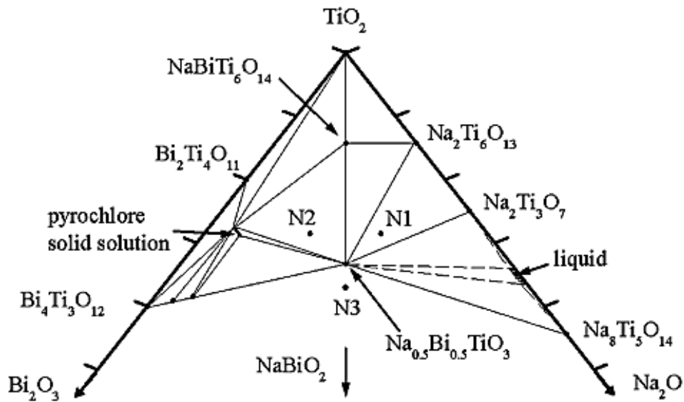
Figure 1: Equilibrium phases in the ternary phase diagram of \text{Bi}_2\text{O}_3\text{-Na}_2\text{O-TiO}_2 at 1000^\circ\text{C} . N1, N2 and N3 correspond to bismuth-, sodium- and titanium-deficient compositions with respect to the stoichiometric \text{Na}_{0.5}\text{Bi}_{0.5}\text{TiO}_3 . [Reproduced with permission from Ref.56 Copyright 2007 Royal Society of Chemistry].
