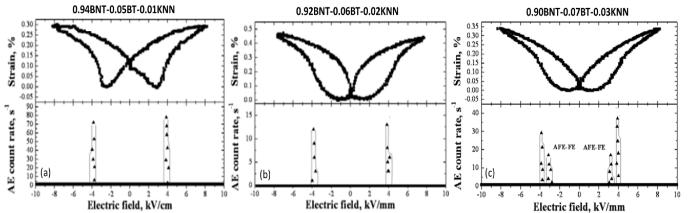
Figure 34. Strain-electric field loops and acoustic emissions of 0.94BNT-0.05BT-0.01KNN (a), 0.92BNT-0.06BT-0.02KNN (b), and 0.90BNT-0.07BT-0.03KNN (c). [Reproduced with permission from Ref.272 Copyright 2009 Elsevier].
