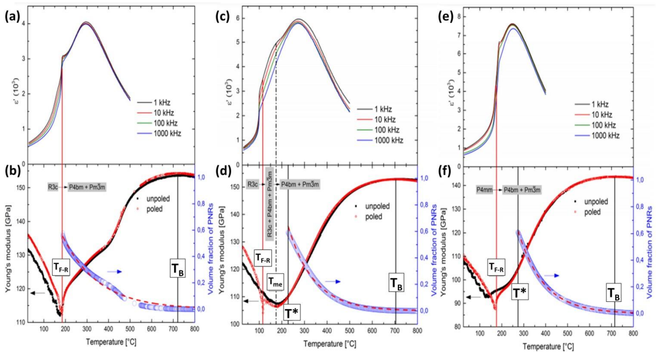
Figure 18. Correspondence between anomalies identified in the temperature dependence of permittivity and Young's modulus for the (1-x)\text{BNT}-x\text{BT} systems: (a)-(b) x=0.03 ; (c)-(d) x=0.06 and (e)-(f) x=0.12 . The dielectric data are relative to poled samples, while mechanical data relative to both unpoled and poled samples. The latter plots contain also the thermal evolution of the volume fraction of polar nanoregions. [Reproduced with permission from Ref.212 https://journals.aps.org/prb/abstract/10.1103/PhysRevB.95.024104 Copyright 2017
