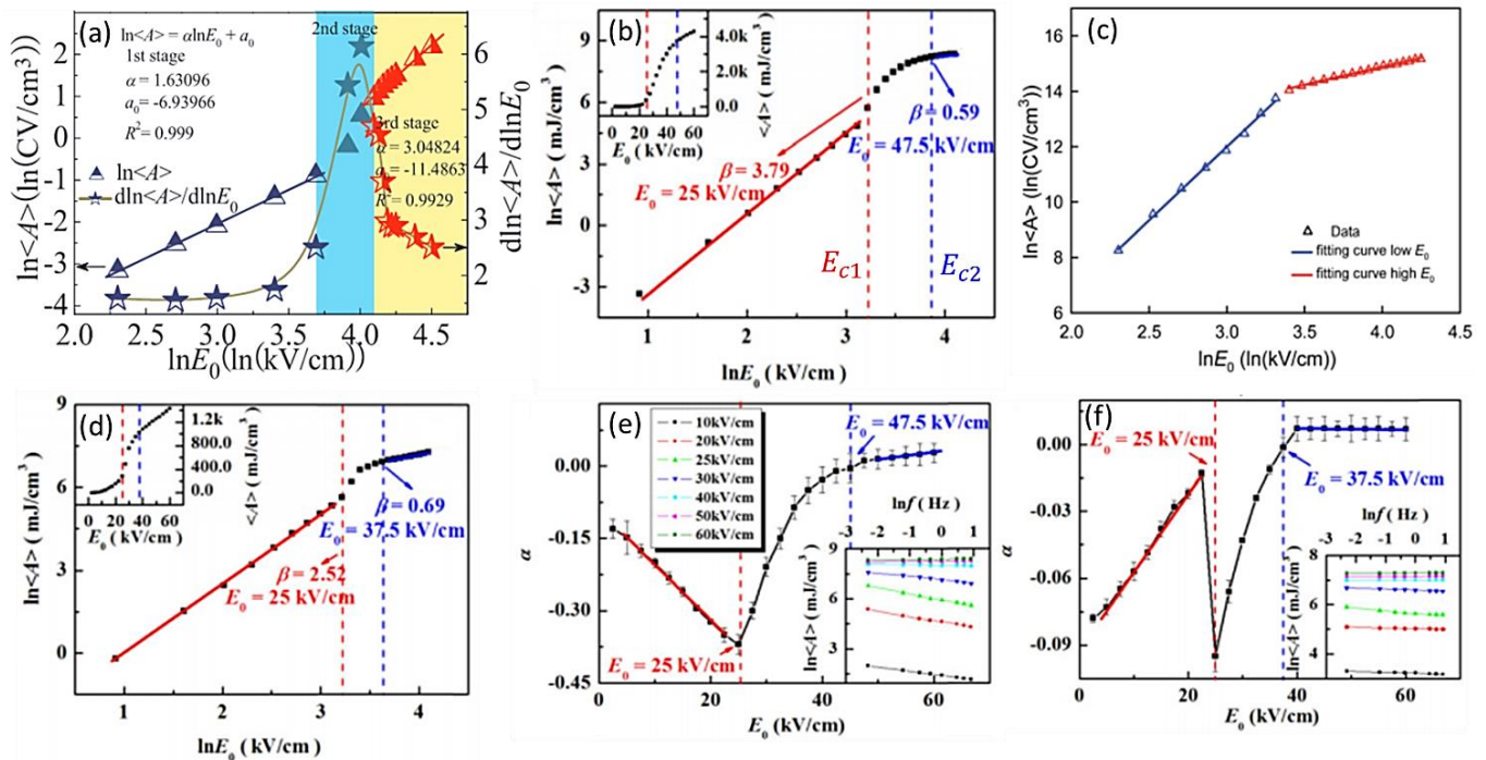
Figure 19. (a)-(d): Dependence of the ferroelectric characteristics on the electric field amplitude and frequency in: (a) BNT at room temperature and 0.1 Hz [Reproduced with permission from Ref.226 Copyright 2019 Elsevier]; (b) 0.94BNT-0.06BT at room temperature and 1 Hz [Reproduced with permission from Ref. 223 Copyright 2014 John Wiley and Sons]; (c) 0.94BNT-0.06BT at room temperature and 0.01 Hz [Reproduced with permission from
