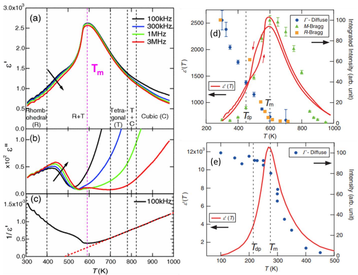
Figure 5. Temperature and dependence of real part (a), imaginary part (b) of dielectric constant and of the inverse of real part of dielectric constant (c) of annealed BNT
