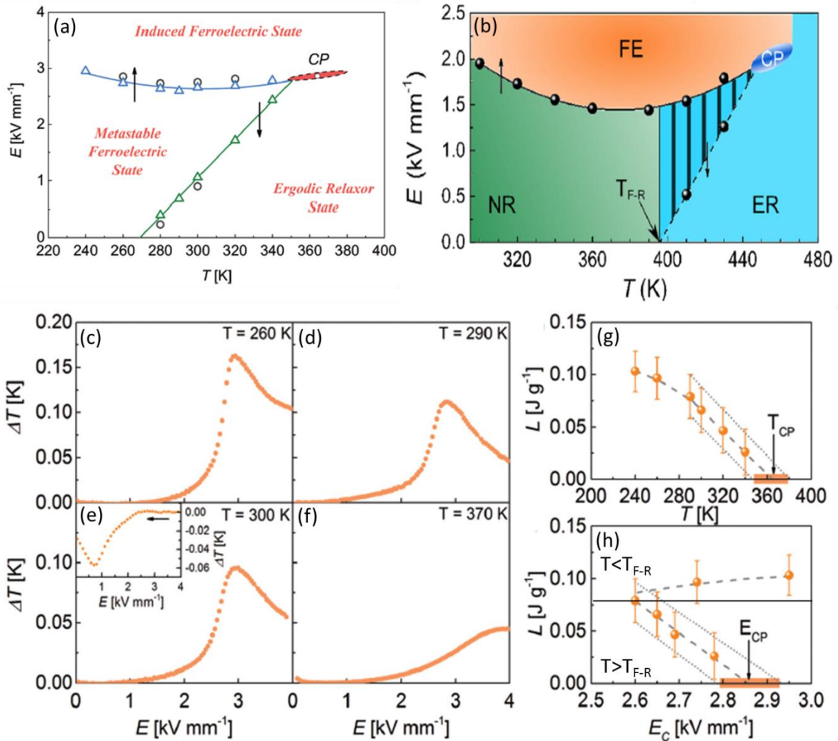
Figure 33. Effects of electric field and temperature on the phase and range of critical points (CP) in 0.75BNT-0.25ST (a) and 0.852BNT-0.028BT-0.12BKT (b). [Reproduced with permission from Ref.263 (Copyright 2016 John Wiley and Sons) and 264 (Copyright 2018 John Wiley and Sons), respectively]. (c)-(f) Temperature changes induced during electrical loading in samples of 0.75BNT-0.25ST ceramics at different external temperatures: 260 K (c), 290 K (d), 300K (e) and 370 K (f). The inset in (e) refers to the temperature changes of the sample during electric field reversal. Extrapolation of critical points from latent heat: critical temperature points T_{CP} (g); critical electric field points E_{CP} (h). [Reproduced with permission from Ref.263 Copyright 2016 John Wiley and Sons].
