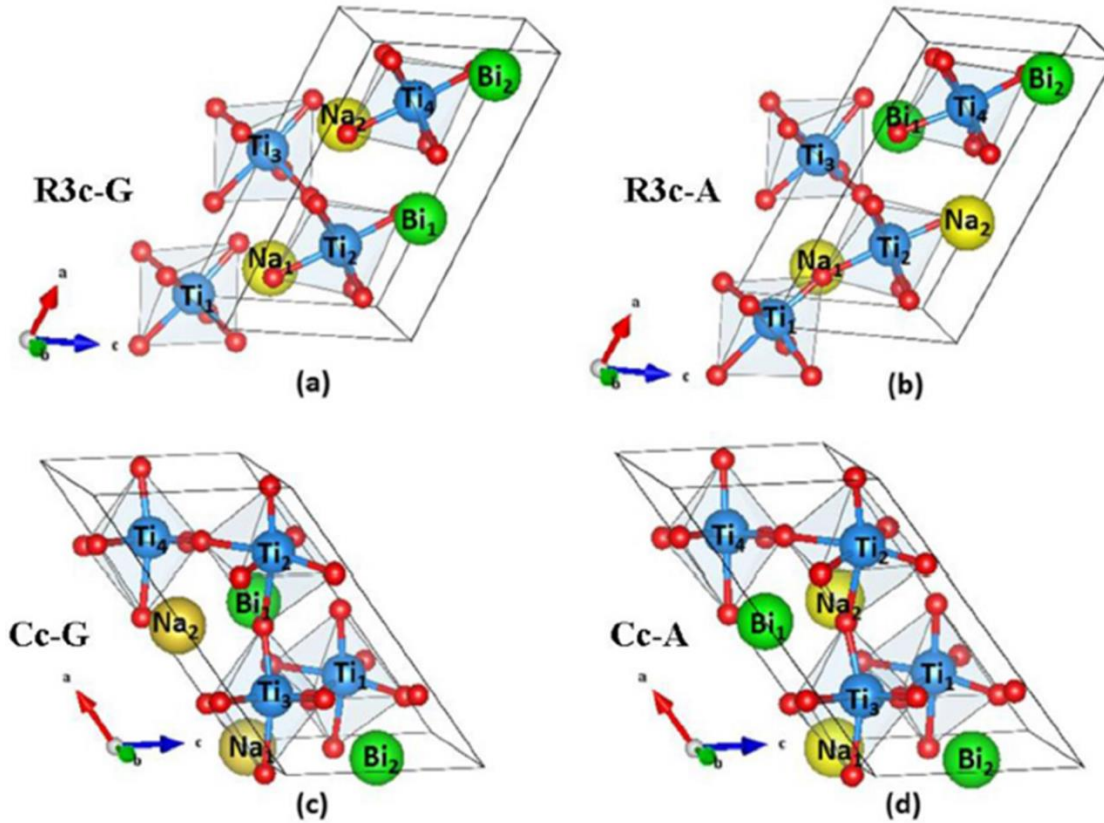
Figure 2. Rhombohedral and monoclinic structures of \text{Bi}_{0.5}\text{Na}_{0.5}\text{TiO}_3 : (a) R3c\text{-G} structure; (b) R3c\text{-A} structure; (c) Cc\text{-G} structure; and (d) Cc\text{-A} structure. [Reproduced from Ref.105 https://aip.scitation.org/doi/10.1063/1.4944473 with the permission of AIP Publishing].
