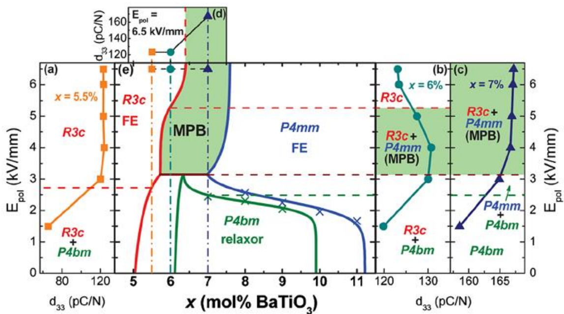
Figure 21. Effect of the electric field on structure and piezoelectric coefficient for different (1-x)\text{BNT}-x\text{BT} compositions across the morphotropic phase boundary range. Green areas indicate the presence of R3c+P4mm MPB. Evolution of d_{33} as a function of the poling field for x=0.055 (a), x=0.06 (b) and x=0.07 (c); (d): evolution of d_{33} as a function of composition in the range 0.055 \leq x \leq 0.07 after poling at 6.5 kV/mm; and (e) variation of the crystal structure as a function of the poling field for different values of x . [Reproduced with permission from Ref.230 https://journals.aps.org/prl/abstract/10.1103/PhysRevLett.109.107602 Copyright
