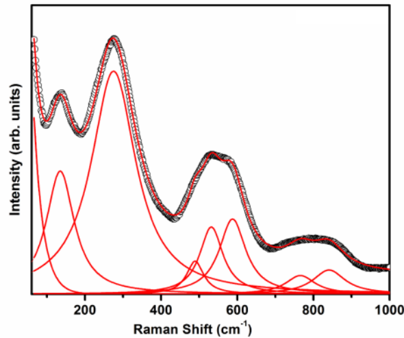
Figure 3: Raman spectrum of \text{Bi}_{0.5}\text{Na}_{0.5}\text{TiO}_3 and deconvolution. [Reproduced from Ref.106 https://iopscience.iop.org/article/10.1088/1361-648X/aaf405/meta with permission from © IOP Publishing].
