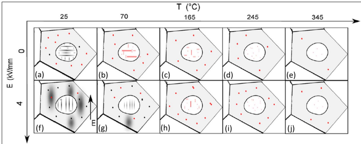
Figure 29. Scheme of temperature and electric field effects on the evolution of the core-shell structure. [Reproduced with permission from Ref.253 Copyright 2015 John Wiley and Sons].
