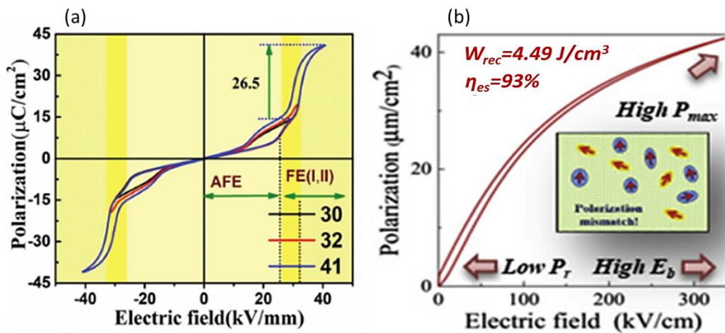
Figure 38. Polarization-electric field hysteresis loops of (\text{Pb}_{0.98}\text{La}_{0.02})(\text{Zr}_{0.55}\text{Sn}_{0.45})_{0.995}\text{O}_3 (a) and 0.6\text{BaTiO}_3-0.4\text{Bi}(\text{Mg}_{1/2}\text{Ti}_{1/2})\text{O}_3 [Reproduced with permission from Ref.299 Copyright 2019 John Wiley and Sons]; (b). [Reproduced with permission Ref.301 Copyright 2020 Elsevier].
