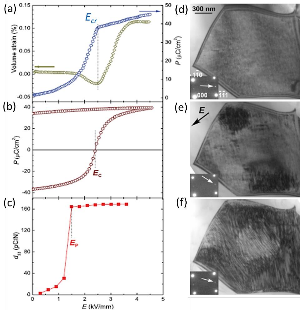
Figure 24. (a) Dependence of volumetric strain and polarization on the electric field on virgin samples; (b) polarization-electric field hysteresis loop; (c) dependence of d_{33} on poling field; (d)-(f) TEM images of a representative grain along the [112] zone-axis under an applied field of 0 kV/mm (d), 1.4 kV/mm (e) and 2.8 kV/mm (f). All plots and images refer to 0.93BNT-0.07BT ceramics. [Reproduced from Ref.231
