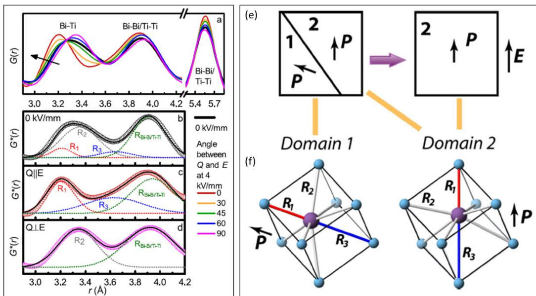
Figure 8. (a) Distribution function G(r) of interatomic distances for Bi-Ti along the [111]_{pc} pseudo-cubic direction and for Bi-Bi/Ti-Ti along the [001]_{pc} pseudo-cubic direction. The black curve indicates the distribution obtained in absence of an applied field ( E=0 kV/mm); the other curves with different colours indicate the distributions obtained during the application of an electric field of 4 kV/mm, for different directions of the scattering vector Q . Following the direction of the black arrow, Q changes orientation from a direction perpendicular to a direction parallel to the applied field; (b)-(d) fitting of the distribution of interatomic distances in absence of an applied field (b) and under an applied field of 4 kV/mm in case Q \parallel E (c) and Q \perp E (d), using three Bi-Ti distances ( R_1 , R_2 and R_3 ) and a single Bi-Bi/Ti-Ti distance all shown in dashed lines; (e) scheme of domain structure evolution from
