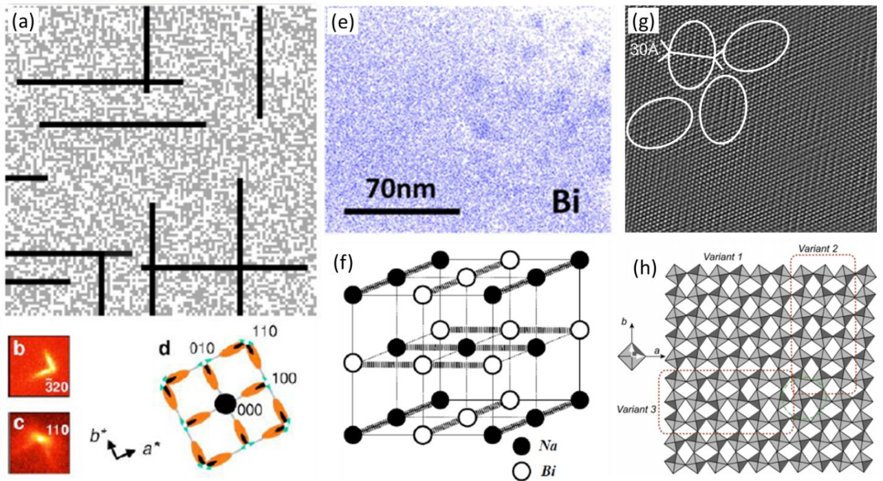
Figure 4. Local structures in BNT: (a) structural model based on Guinier-Preston zones (black bars), immersed in a random distribution of Bi (grey cells) and Na (white cells); (b) asymmetric, L-shaped diffuse scattering around the 3\bar{2}0 reflection; (c) superposition of various asymmetric scattering shown in (d), including asymmetric scattering (black part), thermal scattering (green part) and the large underlying scattering (orange part) for the 110 reflection [reproduced with permission from Ref.109 https://journals.aps.org/prb/abstract/10.1103/PhysRevB.68.014113 Copyright 2003 by the American Physical Society]; (e) distribution of Bi (blue dots) with evident presence of Bi-rich zones [reproduced from Ref.110 with permission from Taylor & Francis https://www.tandfonline.com/doi/abs/10.1080/14786435.2019.1637550?journalCode=tphm20 ]; (f) criss-cross structures [reproduced from Ref.111 https://www.tandfonline.com/doi/abs/10.1080/00150190211198 with permission from Taylor & Francis]; (g) tetragonal nanoplatelets non-homogeneously dispersed within the rhombohedral matrix [reproduced with permission from Ref.112 Copyright 2008 by Elsevier]; (h) coexistence of three variants of (a^- a^- c^+) in-phase tilting [reproduced with permission from Ref.114 Copyright 2012 by John Wiley and Sons].
