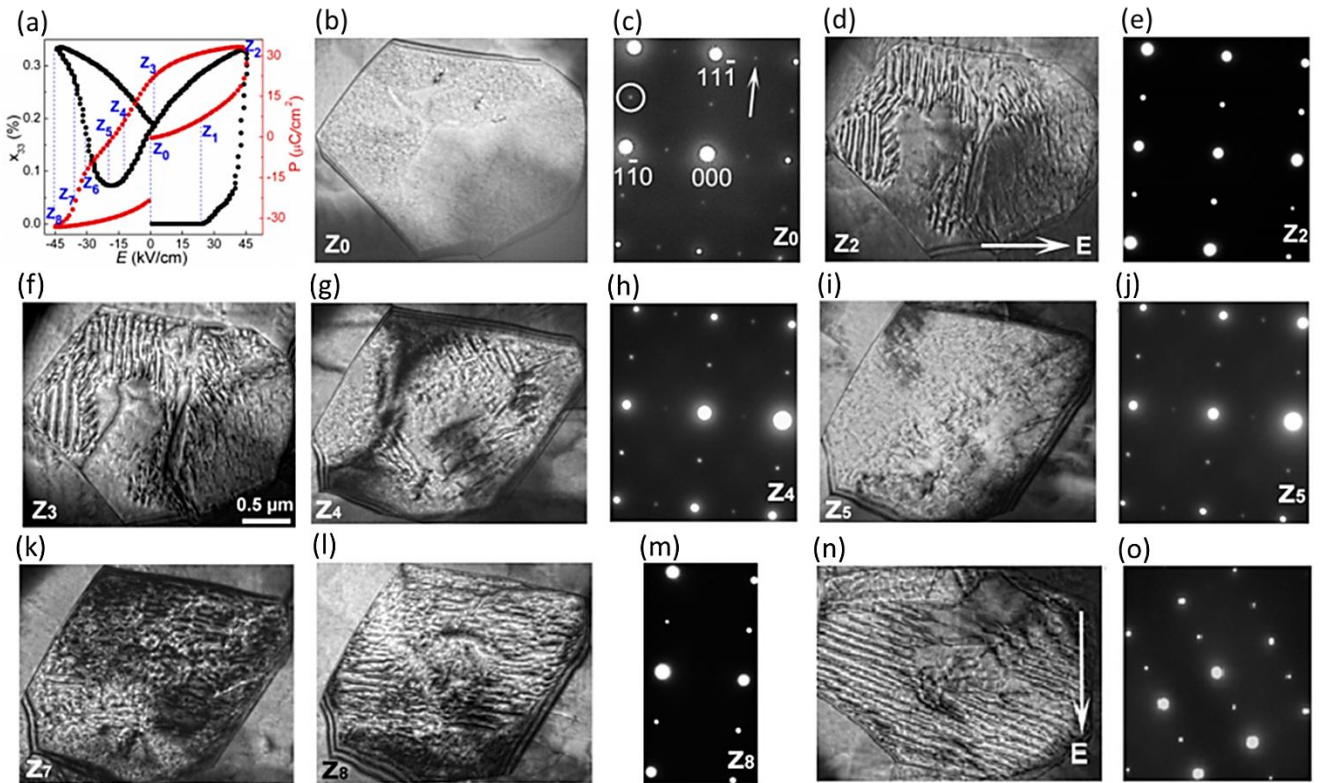
Figure 22. Correlation between the ferroelectric hysteresis and microstructural evolution in [(\text{Bi}_{0.5}\text{Na}_{0.5})_{0.95}\text{Ba}_{0.05}]_{0.98}\text{La}_{0.02}\text{TiO}_3 : (a) polarization- and strain-electric field hysteresis loops; (b)-(m) domain structure and electron diffraction patterns at the different points Z_i along the hysteresis loop; (n), (o) domain structure and electron diffraction pattern after poling.
