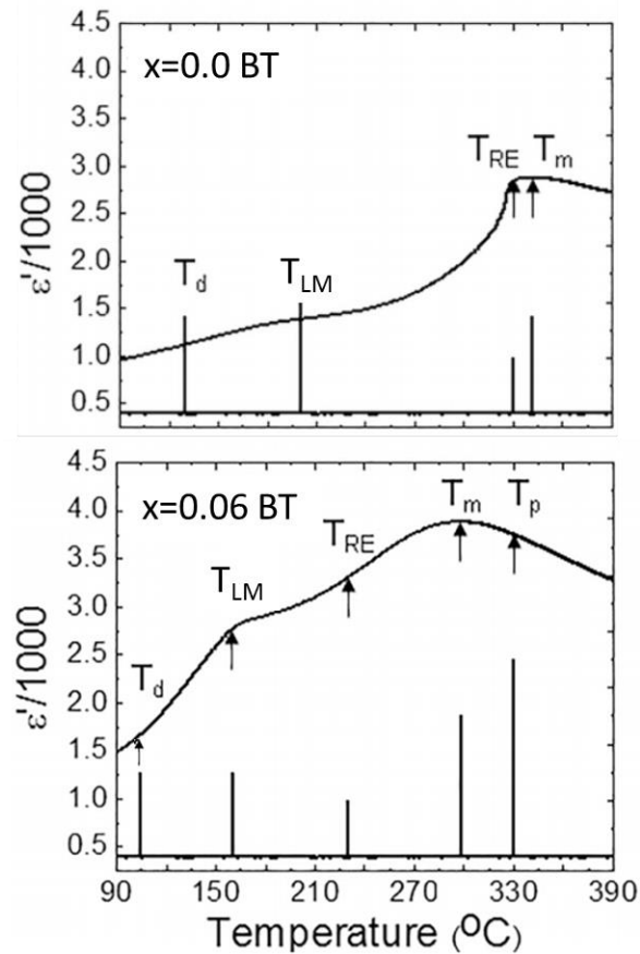
Figure 35. Temperature dependence of dielectric permittivity and identification of characteristic temperature via acoustic emission in single crystals of BNT (a) and 0.94BNT-0.06BT (b). [Reproduced with permission from Ref.273].
