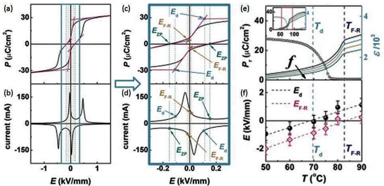
Figure 14. Identification of characteristic fields from hysteresis loops (a)-(d); identification of T_d and T_{F-R} using temperature dependence of remnant polarization and permittivity (e) and characteristic fields E_d and E_{F-R} (f). [Reproduced with permission from Ref.208 Copyright 2019 Elsevier].
