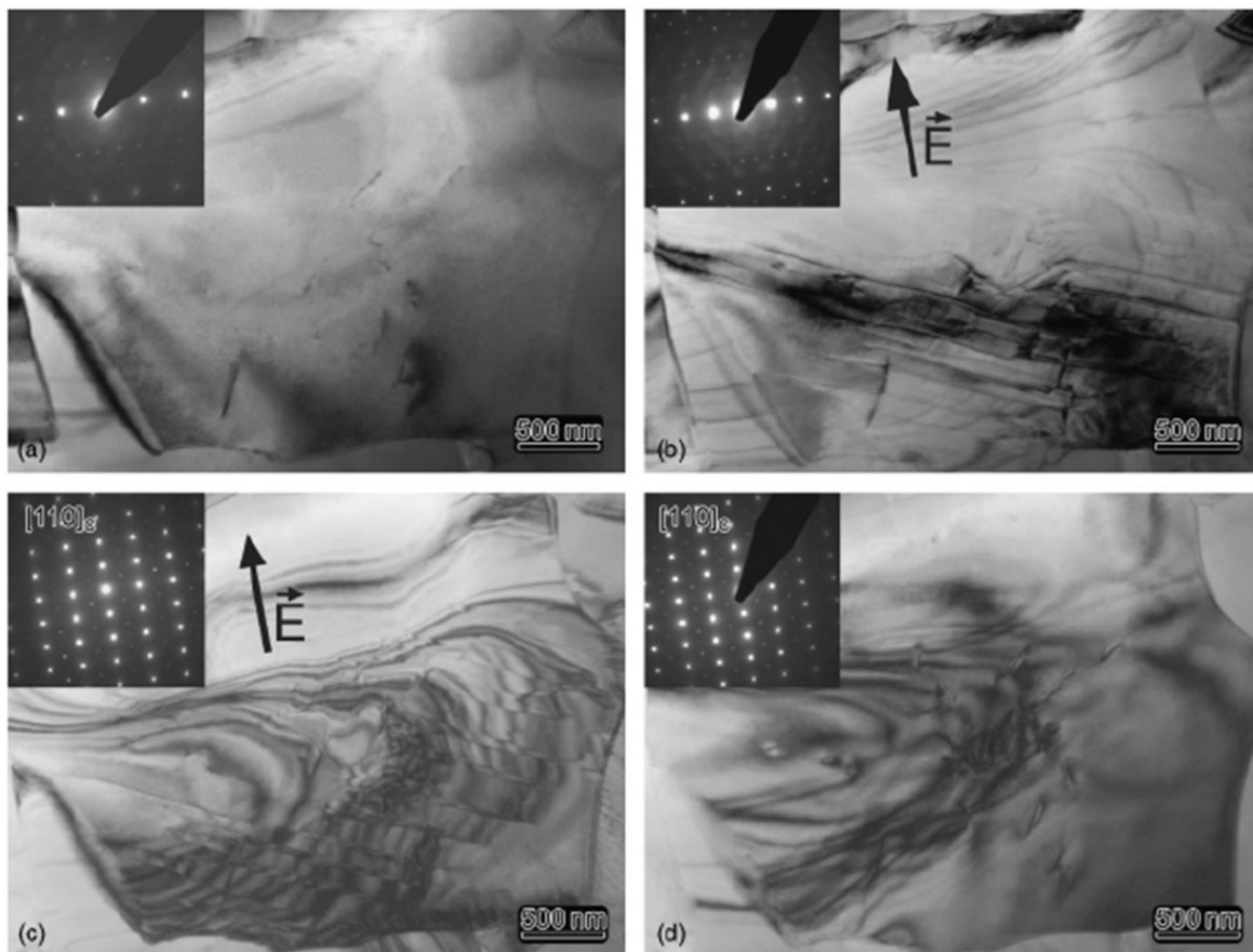
Figure 23. Evolution of microstructure and electron diffraction patterns in a grain of 0.91BNT-0.06BT-0.03KNN during the application of an electric field: (a) before applying the electric field no domains are present; (b), (c) at a nominal field of 25 kV/cm (actual field of about 50 kV/cm) lamellar domains are present; (d) after removing the electric field.
