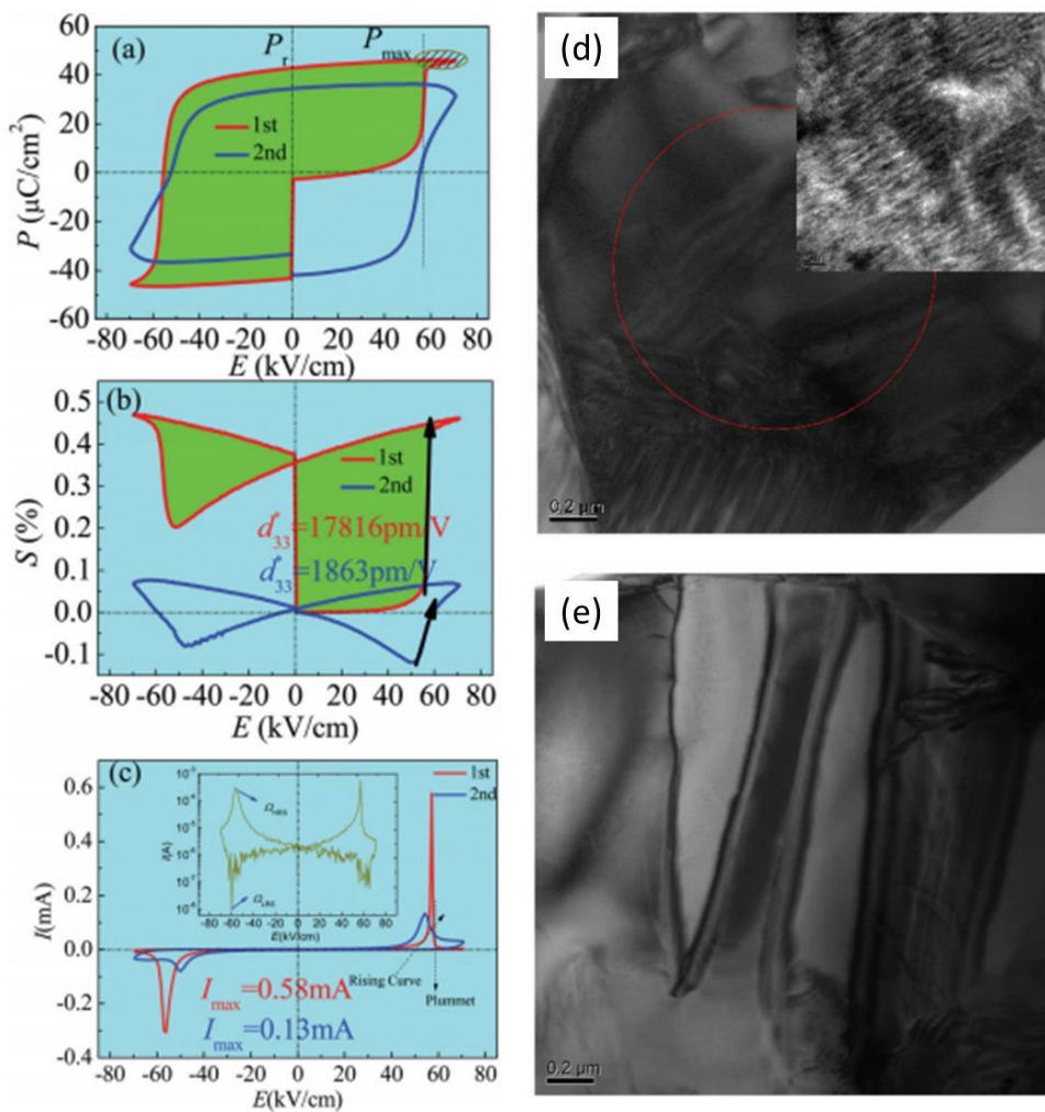
Figure 9. Hysteresis loops obtained during two successive electric field cycles: (a) polarization-electric field; (b) strain-electric field; (c) current-electric field; domain structure in unpoled (d) and poled (e) state. [Reproduced with permission from Ref.103 Copyright 2019 Royal Society of Chemistry].
