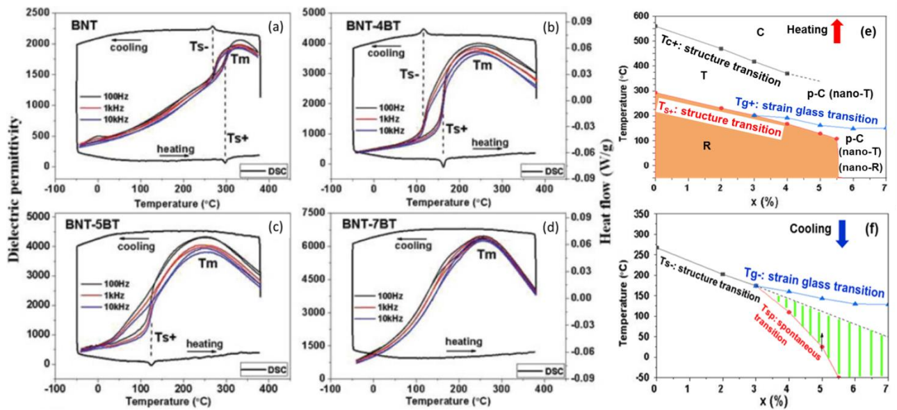
Figure 16. (a)-(d): temperature dependence of dielectric permittivity and differential scanning calorimetry thermograms of BNT (a), 0.96BNT-0.04BT (b), 0.95BNT-0.05BT (c), and 0.93BNT-0.07BT (d). [Reproduced from Ref.209 https://www.tandfonline.com/doi/pdf/10.1088/1468-6996/14/3/035008?needAccess=true with permission from Taylor & Francis]; (e)-(f) Phase diagrams of (1-x) BNT- x BT ( 0 \leq x \leq 0.07 ) during heating (e) and cooling (f). [Data obtained from the authors of Ref.209].
