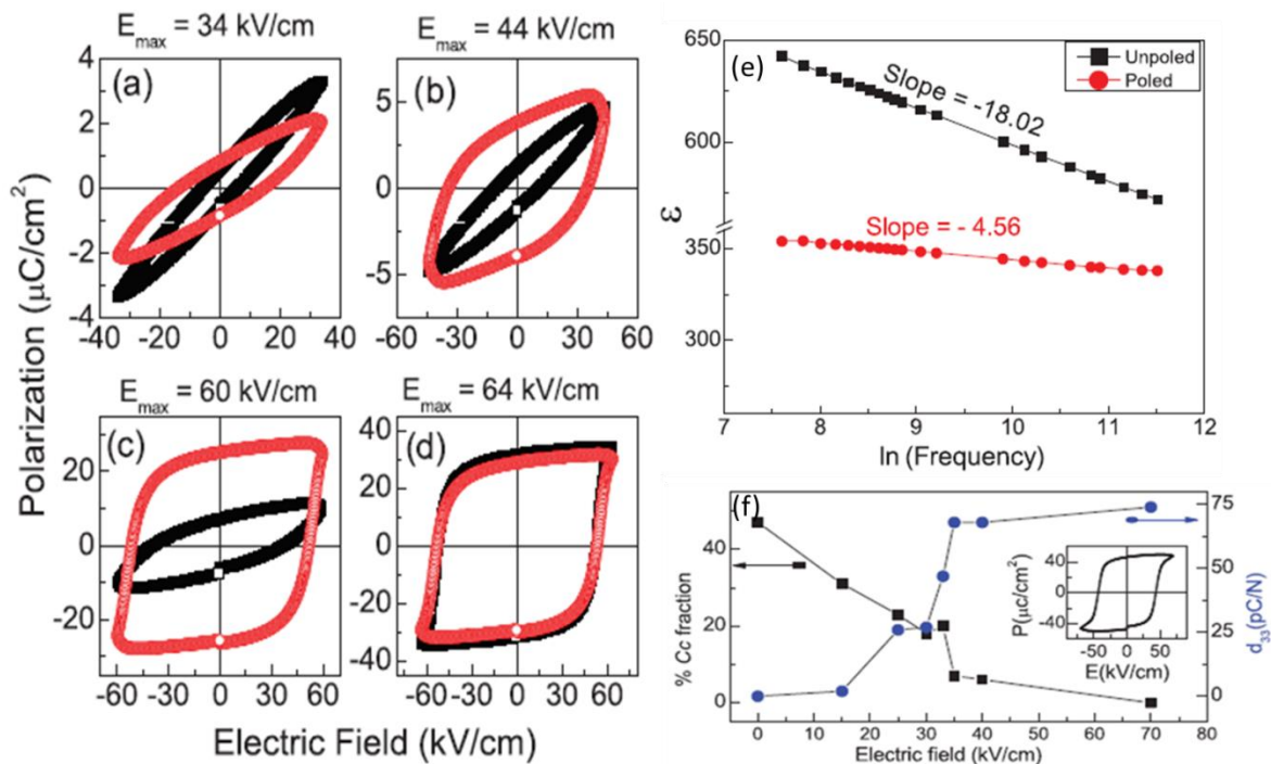
Figure 6. (a)-(d) P-E loops obtained at different electric field amplitudes. Black curves represent the loops obtained on initially unpoled ceramics with increasing the maximum applied field. Red curves represent the loops obtained by decreasing the maximum field applied on the ceramic undergone the electrical history represented by the black curves sequence [Reprinted with permission from Ref.119
