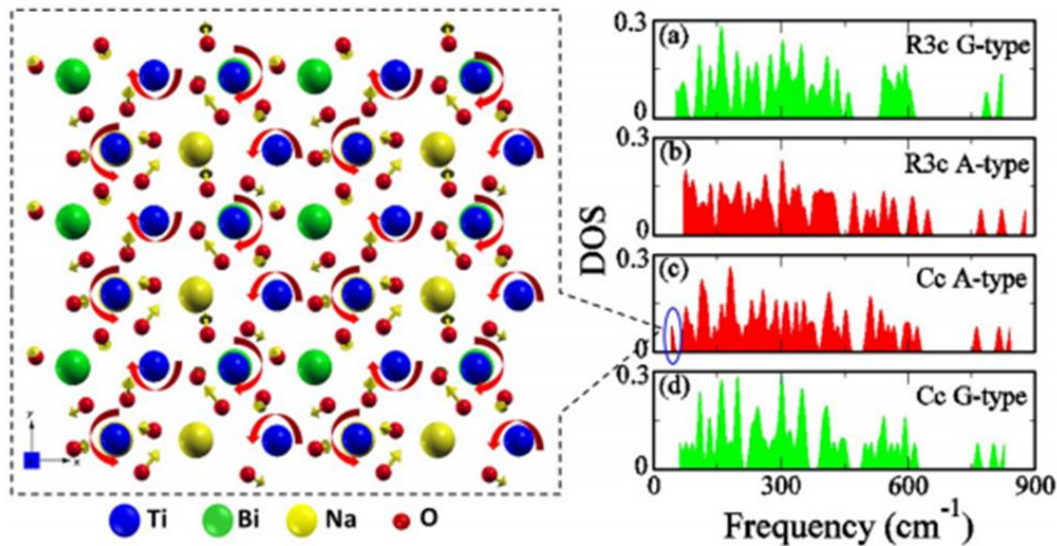
Figure 7. Vibrational density of states in different structures: (a) R3c-G , (b) R3c-A , (c) Cc-A , and (d) Cc-G . The left inset shows a schematic representation of the softest phonon mode identified in the Cc-A structure. [Reproduced from Ref.105 https://aip.scitation.org/doi/10.1063/1.4944473 with the permission of AIP Publishing].
