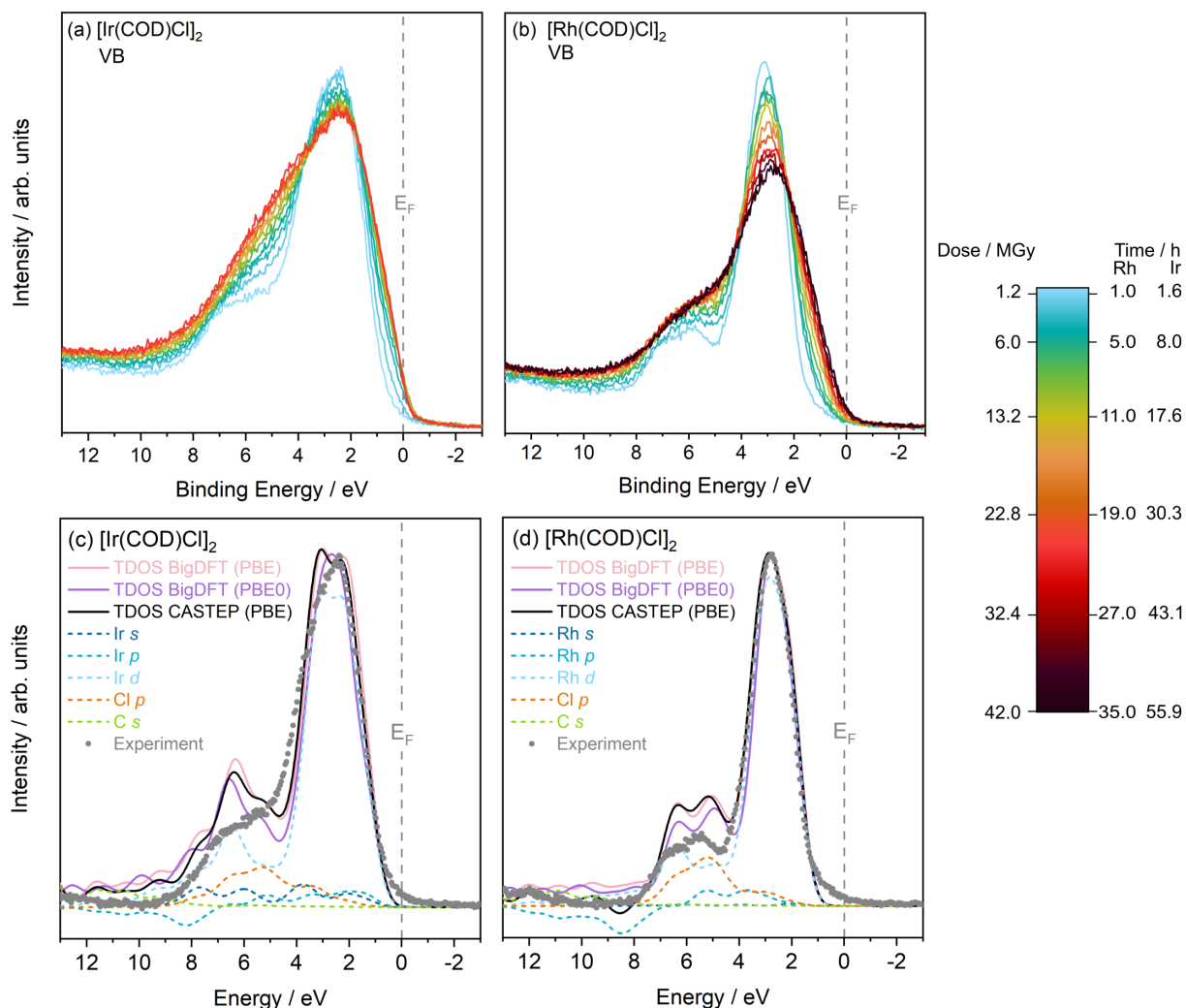
Figure 8: Electronic structure of the [M(\text{COD})\text{Cl}]_2 catalysts. (a) and (b) Valence band X-ray photoelectron spectra of [\text{Ir}(\text{COD})\text{Cl}]_2 and [\text{Rh}(\text{COD})\text{Cl}]_2 , respectively. The legend includes the measurement time as well as the calculated X-ray dose as Average Dose Whole Crystal (AD-WC) from RADDOSE-3D. (c) and (d) Broadened and photoionisation cross section corrected total (TDOS) and projected (PDOS) density of states, calculated using the CASTEP code with the PBE functional, compared to the initial XPS data for [\text{Ir}(\text{COD})\text{Cl}]_2 and [\text{Rh}(\text{COD})\text{Cl}]_2 , respectively. Only the states with significant contributions to the intensity are displayed. The TDOS is included for both the CASTEP PBE calculations as well as for the BigDFT PBE and PBE0 calculations for comparison. The Fermi energy E_F at 0 eV is indicated in all subfigures.
