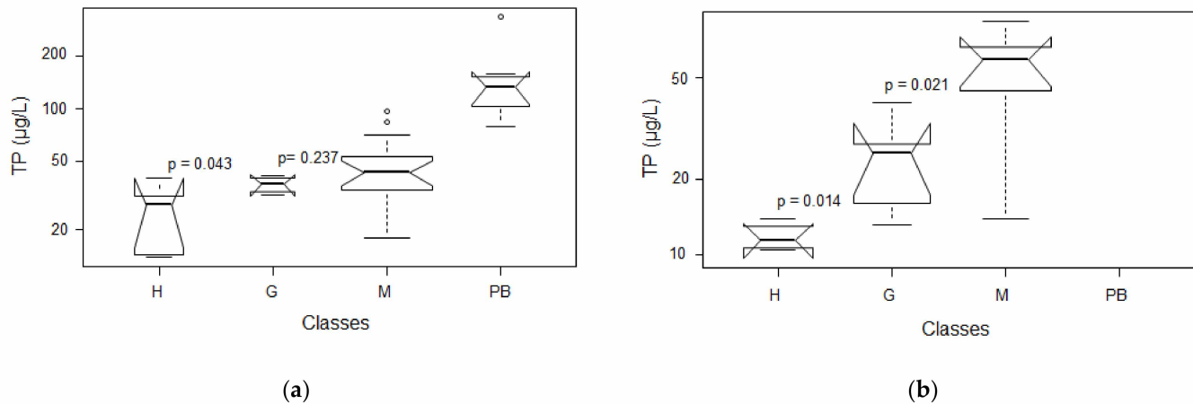
Figure 3. Box plots showing range of Total Phosphorus (TP, \mu\text{g/L} ) concentrations by ecological classes (H: High, G: Good, M: Moderate, PB: Poor-Bad) in (a) Greek Shallow Natural Lakes (GR-SNL); (b) Greek Deep Natural Lakes (GR-DNL). The width of boxes is proportional to number of records in class. The p -values represent the significance of Wilcoxon test results.
