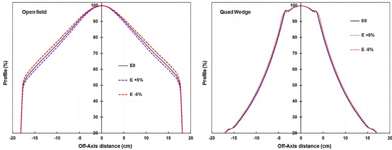
FIG. 3. Diagonal profiles measured with an ionization chamber profiler (ICA) with open field (left) or with quad wedge atop the ICA (right) for nominal beam energy (E: 0%), and energy changes +5% (E: +5%) and -5% (E: -5%) from nominal energy. The source-to-surface (SSD) is 90 cm, depth d_{max} , and the field size is 28 \times 28 \text{ cm}^2 .
