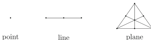
Fig. 3 Hypergraphs of the examples from Fig. 2
