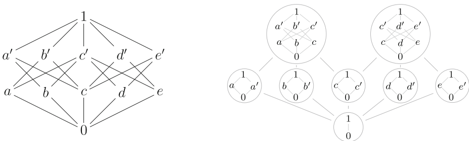
Fig. 1 The orthoalgebra on the left is constructed from gluing together two Boolean algebras \{0, a, b, c, a', b', c', 1\} and \{0, c, d, e, c', d', e', 1\} . The orthogonal sum \oplus is the union of the orthogonal join operations of these Boolean algebras. On the right is the Hasse diagram of its poset of Boolean subalgebras
