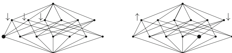
Fig. 5 Direction for a distinguished atom in a 16-element Boolean algebra
