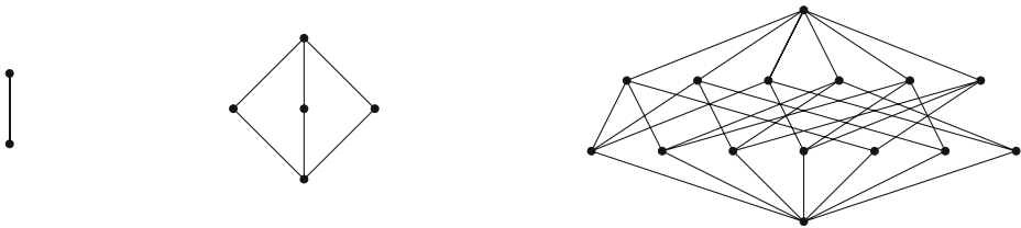
Fig. 2 Hasse diagrams of the posets BSub(A) for Boolean algebras A with 4, 8, and 16 elements. A Boolean algebra with 4 elements has two subalgebras: \{0, 1\} , and itself. A Boolean algebra A with 8 elements has five subalgebras: \{0, 1\} , three subalgebras \{0, a, a', 1\} for a \in A \setminus \{0, 1\} , and A itself. A Boolean algebra with 16 elements has a more complicated structure of subalgebras, containing subalgebras with 2, 4, 8, and 16 elements
