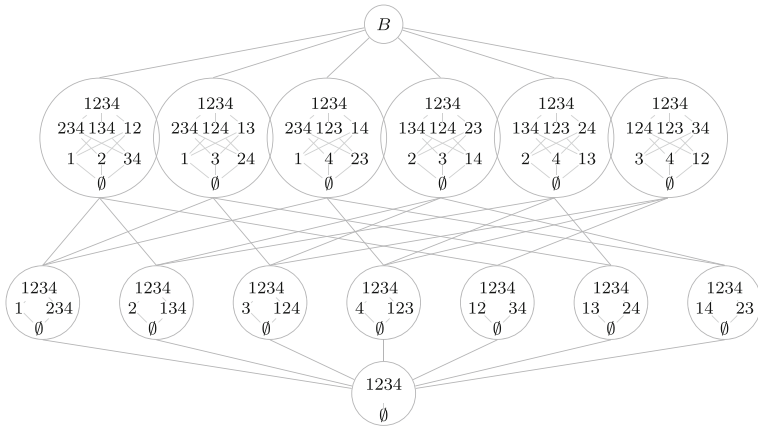
Fig. 4 The poset of subalgebras of a 16-element Boolean algebra
