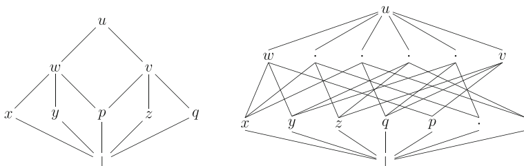
Fig. 6 A part of the Hasse diagram of the shadow from the proof of Lemma 5.6 (two possible partial diagrams of the same situation)
