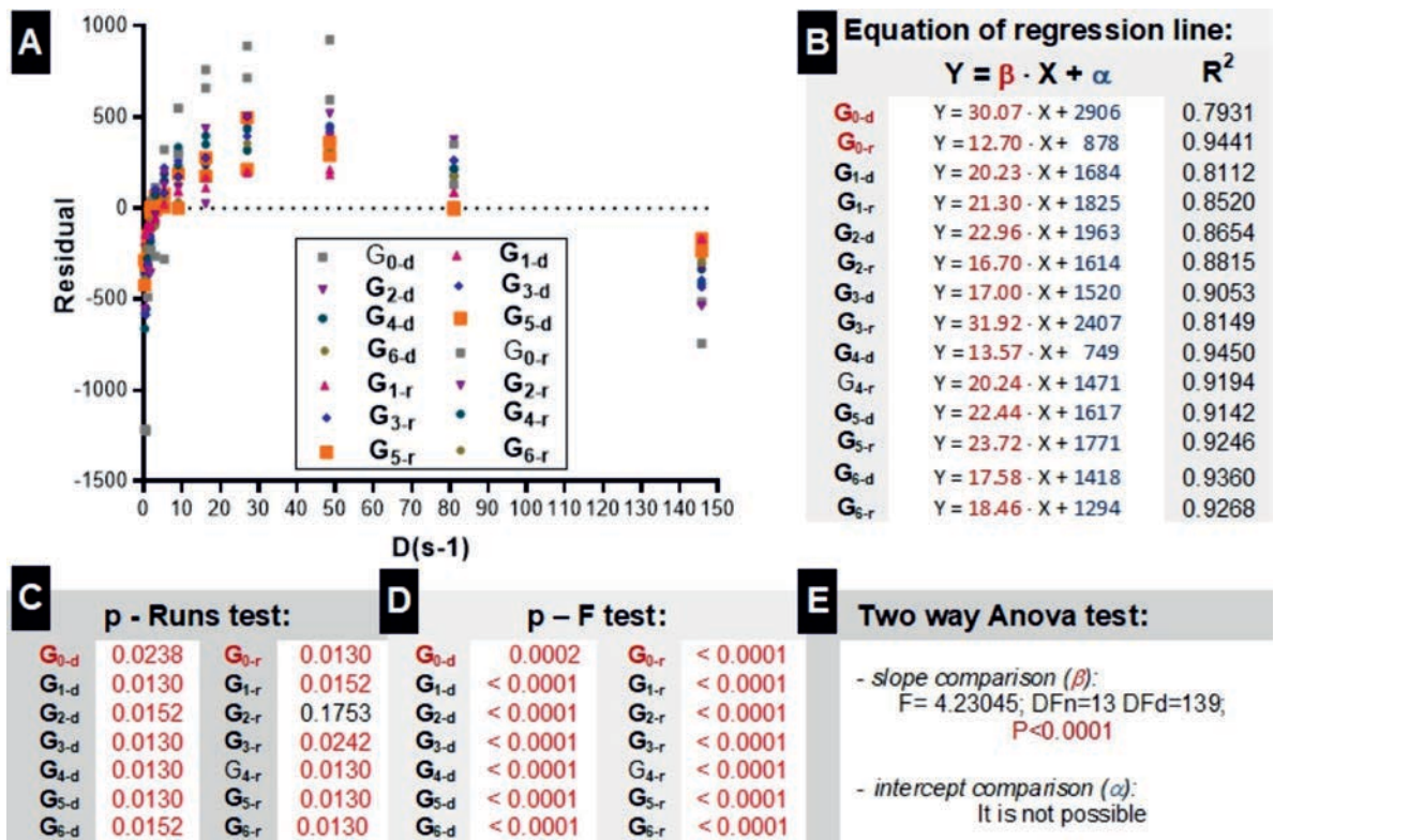
FIGURE 3. Analysis of flow curves by linear regression: residuals (A), equation of regression lines (B), deviation from linearity (C), deviation from zero (D), results of the variance test (E)
