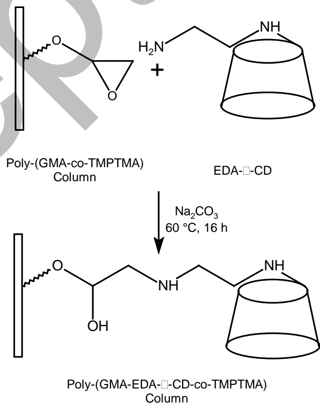
Fig 3. Preparation of poly-(GMA-EDA-β-CD-co-TMPTMA)
