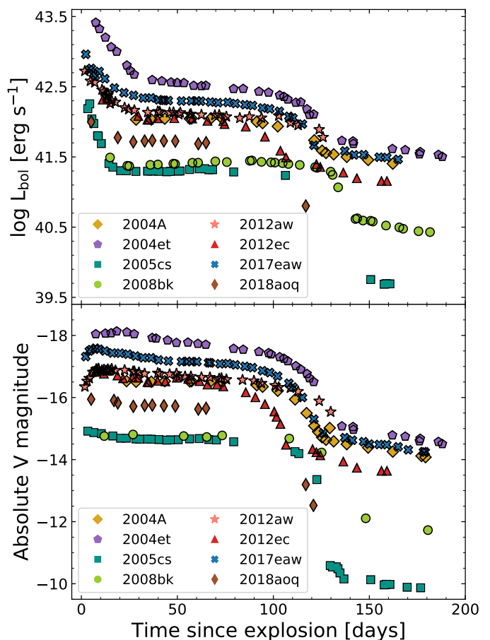
Fig. 3. Bolometric LCs (top panel) and absolute V -band LCs (bottom panel) of SN 2017eaw and SN 2018aoq in comparison to well-studied SN 2004A, SN 2004et, SN 2005cs, SN 2008bk, SN 2012ec, and SN 2012aw. Absolute curves were computed using the distances and reddening in Table 1 of MB19, except in the case of SN 2004et for which we use the new estimates of the distance (see text).
