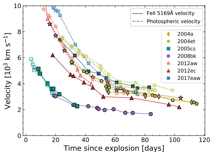
Fig. 13. Comparison between observed Fe II velocities (filled markers, solid lines) and photospheric velocities (open markers, dashed lines) inferred from H\beta velocities through the polynomial relation from Jones et al. (2009) for each SN in our sample. Errors are not plotted for better visualisation.
