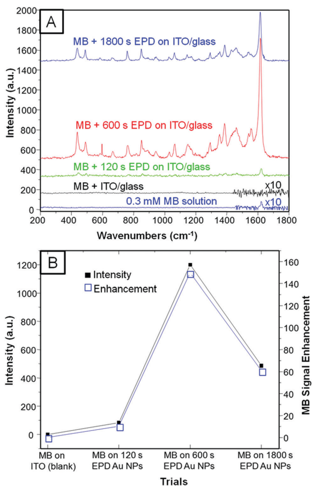
Fig. 3 Selected Raman spectra of 0.3 mM MB blank sample and the three different quick SERS tests based on 120, 600, and 1800 s EPD of Au NPs on ITO/glass (A). Plot shows a three-entry plot of intensity vs. MB signal enhancement vs. all the trials performed in this work including the blank (B). Spectra in A are off-set for a better comparison.
