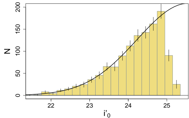
Figure 13. Luminosity function of the GC candidates. The vertical bars symbolize the error corresponding to each bin, and the solid line represents the Gaussian fit.
