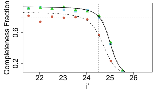
Figure 2. Completeness fraction for the inner region (dots), medium region (squares) and external region (triangles). Each region has its corresponding fit plotted in dot-dashed, solid and dotted, respectively. The dashed line shows the chosen limit.
