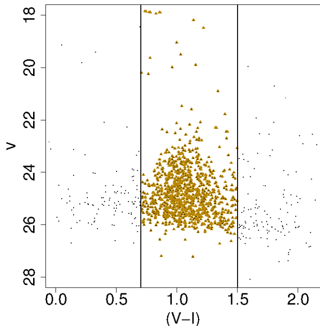
Figure 5. Colour-magnitude diagram for the point-source objects detected on the WFPC2 field (circles). The triangles indicate those that fulfill the colour criteria described in the text to be considered GC candidates.
