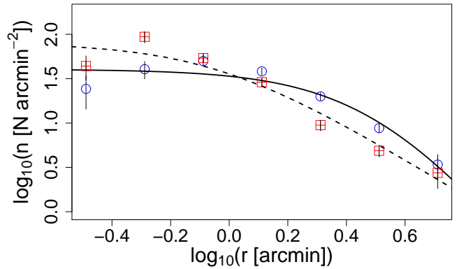
Figure 10. Projected radial distribution for the entire GC population (top panel), both corrected for completeness (squares) and without applying the corrections (circles), and for the red (squares) and blue (circles) sub-population (lower panel). For the entire population, the solid line shows a Hubble function fit, while the dashed line shows a power-law fit. In the case of the sub-populations, they both have Hubble function fits, the solid line depicts the corresponding to the blue GCs and the dashed line, the one for the red GCs. The dotted line depicts the background level.
