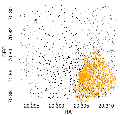
Figure 9. Spatial distribution of the GMOS sources (dots) and the WFPC2 sources (triangles), obtained with SExtractor.
