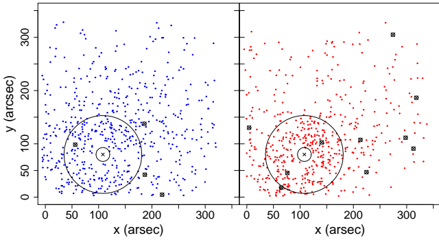
Figure 8. Projected spatial distributions for the blue (left panel) and red (right panel) GC candidates. The circles signal the region used for the azimuthal analysis in Section 4.3. The crossed-out circles depict the location of UCD candidates.
