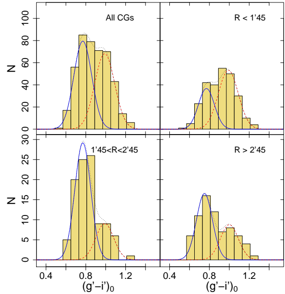
Figure 7. Colour distribution diagrams corresponding to the entire population in the top left panel, and to rings at different galactocentric distances in the following panels, moving from the inner region (top right) to the outer region (bottom right). The blue solid and the red dashed lines represent the gaussian fits corresponding to the metal-poor and to the metal-rich subpopulation respectively. The dotted black line shows the sum of both functions.
