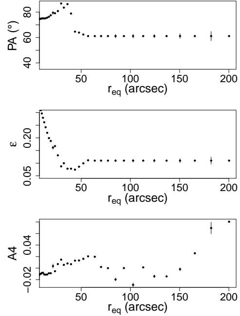
Figure 15. Upper panel: position angle of the elliptical isophotes versus effective radius. Middle panel: ellipticity of the elliptical isophotes versus effective radius. Lower panel: Parameter A_4 versus effective radius.
