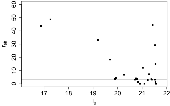
Figure 6. Distribution of the effective radius of all point-like sources with magnitudes brighter than the assumed limit for UCD candidates, against the GMOS i'_0 magnitude. The solid line indicates r_{\text{eff}} = 3 pc, the typical value for GCs (Jordán et al. 2007).
