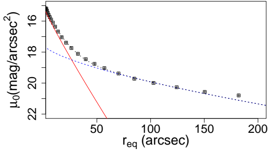
Figure 14. Surface brightness profile of NGC 6876 in i'_0 . The solid line and the dashed line represent the inner and outer components, respectively, while the dotted line represents the sum of both.
