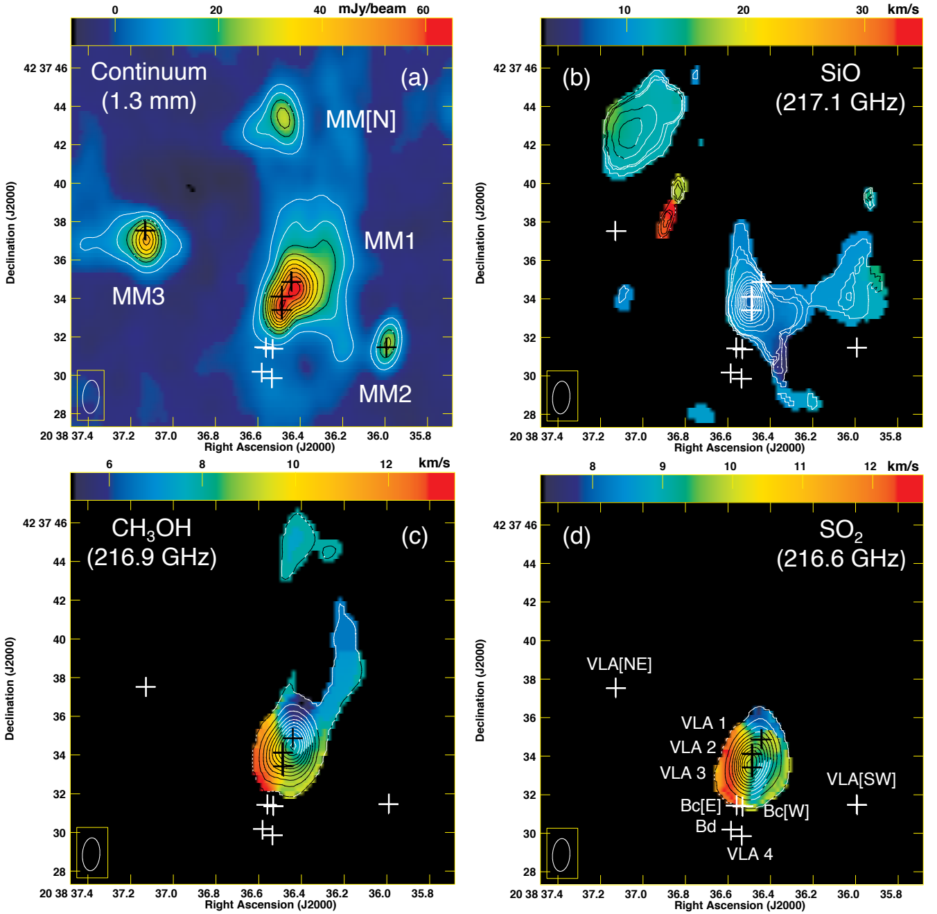
Figure 3. (a) Colour image and contour map of the continuum emission at 1.3 mm. Contour levels are 1, 2, 3, 4, 5, 6, 7, 8, 9, 10 \times 6.1 mJy beam ^{-1} . The mm sources MM1, MM2, and MM3 are labeled (nomenclature by Minh et al. 2010). A new mm source detected with ALMA \sim 9 arcsec north from MM1 is labeled as MM[N]. Crosses indicate the positions of the radio continuum sources at cm wavelengths identified with the VLA (this work). (b) Contour map of the integrated intensity and velocity field colour image (moment of order 1) of the SiO (217.1 GHz) line. Contour levels are 0.4, 0.8, 1, 2, 3, 4, 5, 6, 7, 8, 9, 10 \times 0.27 Jy beam ^{-1} km s ^{-1} . (c) Same as the previous panel but for the CH 3 OH (216.9 GHz) line. Contour levels are 0.1, 1, 2, 3, 4, 5, 6, 7, 8, 9, 10 \times 0.6 Jy beam ^{-1} km s ^{-1} . (d) Same as the previous panel but for the SO 2 (216.6 GHz) line. Contour levels are 0.1, 1, 2, 3, 4, 5, 6, 7, 8, 9, 10 \times 0.8 Jy beam ^{-1} km s ^{-1} . Primary beam corrections have not been applied to these images, given that the mm cores are detected at the edge of the ALMA primary beam (FWHM \approx 27 arcsec; see Section 3.2). Assuming that the ALMA primary beam can be approximated by a Gaussian function, the intensities given in these images should be corrected by factors of \sim 4, 10, 2, and 1.4 at the positions of MM1, MM2, MM3, and MM[N], respectively.
