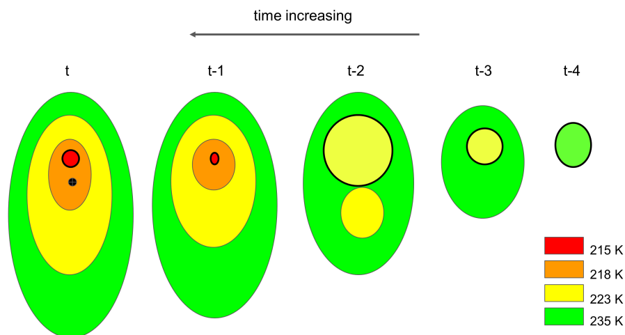
Figure 3. Simplified scheme of adaptive threshold technique. The black dot represents the ERPF centroid location and filled contours different temperature clusters. Bold lines denote the temperature threshold at each time.
