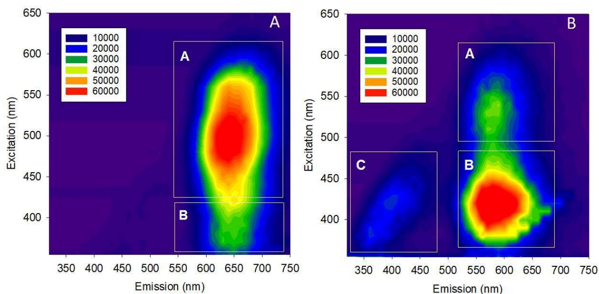
Fig 2. Excitation-Emission matrix of aqueous suspension of BSA-capped GNC under Argon and air saturation, figures (A) and (B), respectively. Box A shows the zone of excitation and emission of the \text{Au}_{25} nanoclusters; box B represents the energy transfer between the spectra of smaller and \text{Au}_{25} clusters, while box C shows the fluorescent properties of the smaller nanoclusters.
