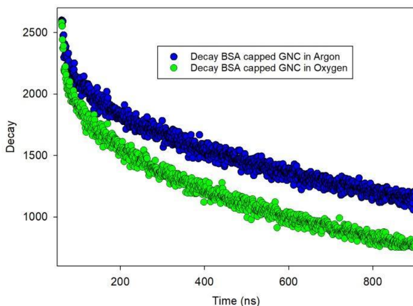
Fig 4. Time Decay BSA-capped GNC in presence (green circles) and absence (blue circles) of oxygen. The PL traces detected at 640 nm upon 341 nm excitation
