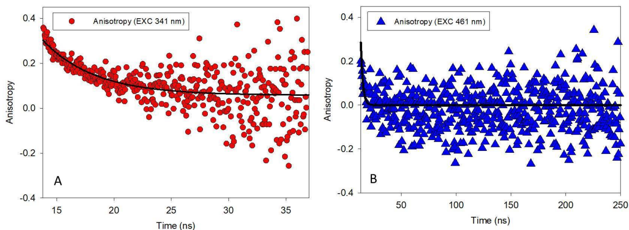
Fig 5. Time-domain anisotropy decay of BSA-capped GNC. Graph (A) exciting with 341 nm and Graph (B) exciting with 461 nm. The emission was detected at 640 in both cases.
