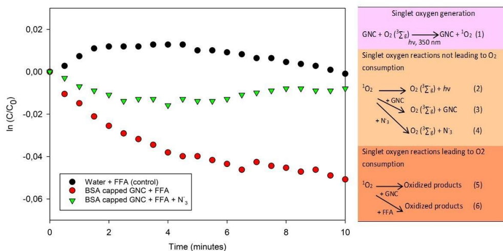
Fig 8. Molecular oxygen consumption during irradiation at 350 nm of air-saturated aqueous suspensions of water + FFA (black circles), BSA-capped GNC with 10^{-3} M FFA (red circles) and BSA-capped GNC with 10^{-3} M FFA and 10^{-2} M azide (green triangles). The reactions in each experiment are also shown in the panel at the right.
