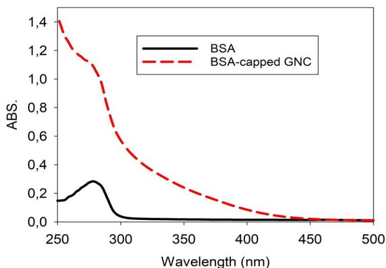
Fig 1. UV-Vis spectra of BSA (black line) and BSA-capped GNC (red dotted line) adjusted to a final concentration of 0.5 mg/mL of BSA protein in PBS buffer 10 mM pH = 7.4
