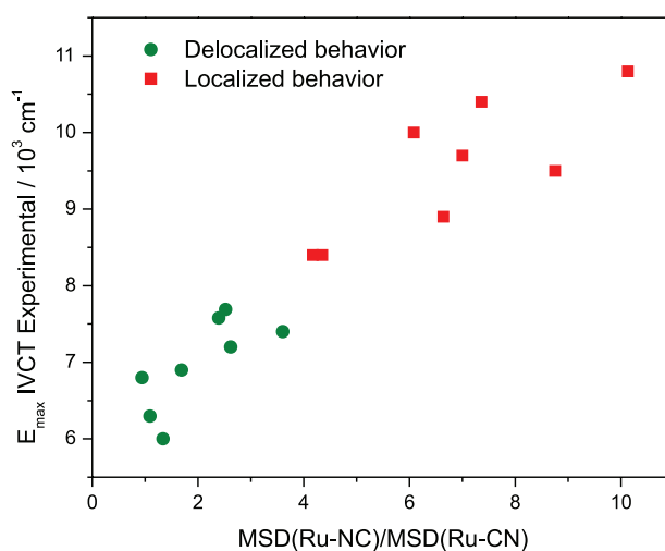
Figure 3. Correlation of experimental IVCT energies with ruthenium Mulliken spin densities ratio.
