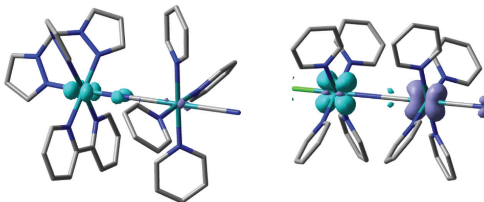
Figure 5. EDDM (0.004 a.u.) of the most intense NIR transition for the doublets 2 3+ (left) and 13 2+ (right) ions calculated in MeCN. Purple indicates a decrease in charge density, while cyan indicates an increase.
