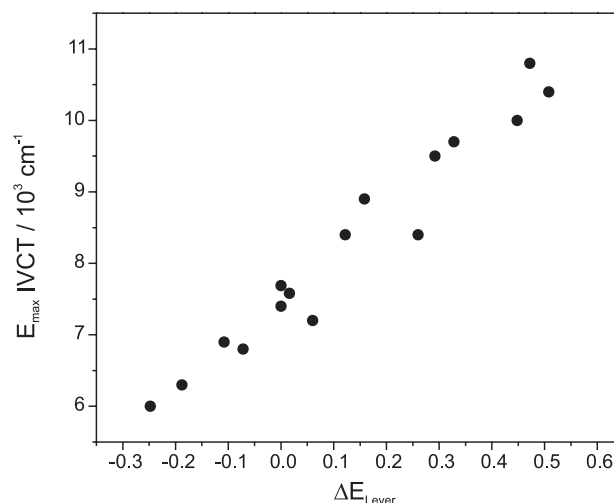
Figure 1. Correlation between E_{max} IVCT and difference of ruthenium redox potentials estimated using Lever parameters.
