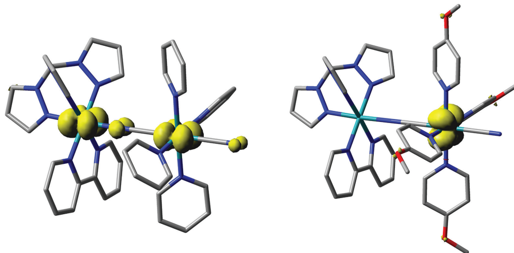
Figure 4. Spin density isosurface plot (0.004 a.u.) for 2^{3+} (left) and [\text{Ru}^{\text{II}}(\text{tpm})(\text{bpy})(\mu\text{-NC})\text{Ru}^{\text{III}}(\text{MeOpy})_4(\text{CN})]^{3+} (right) in MeCN showing different orientation of unpaired electron.
