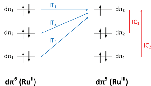
Scheme 2. IT and IC transitions in d\pi^6 - d\pi^5 mixed-valence systems such as \text{Ru}^{\text{II}}\text{-L-Ru}^{\text{III}} complexes.
