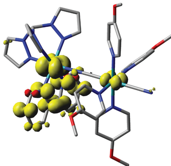
Figure 6. Spin density isosurface plot (0.004 a.u.) for the lowest-lying triplet state of [\text{Ru}^{\text{II}}(\text{tpm})(\text{bpy})(\mu\text{-NC})\text{Ru}^{\text{II}}(\text{MeOpy})_4(\text{CN})]^{2+} ion in DMSO.
