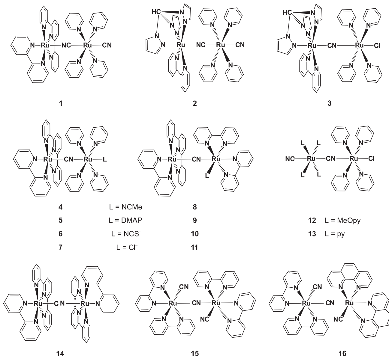
Scheme 1. Structure of targeted molecules (DMAP: 4-dimethylaminopyridine, MeOpy: 4-methoxypyridine, py: pyridine).
