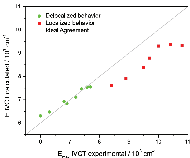
Figure 2. Correlation of calculated IVCT energies with experimental data.
