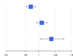
Fig. 2 Association results of rs72824905-G with dementia by-proxy and longevity by-proxy analysis in the UK Biobank. * P values < 0.05. The figure shows the odds-ratio (box) of the rs72824905-G with the 95% confidence intervals (whiskers)
