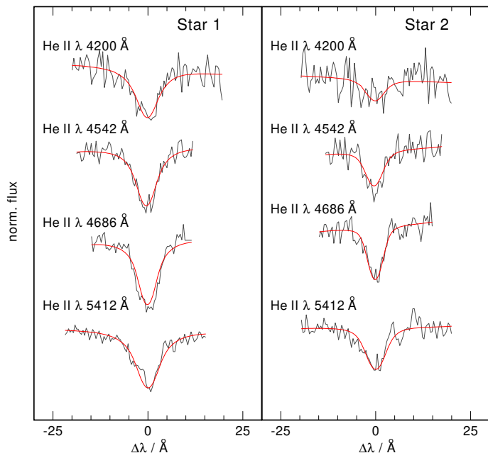
Fig. 4. He II lines of the decomposed OSIRIS spectrum #2 (gray) shown along with the best fit TMAP models (red).
