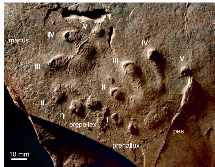
Fig. 15. The track Amphisauropus Haubold, 1970, NMMNH P-37922, central New Mexico, USA, Abo Formation, Cisuralian, left manus and pes imprint, convex hyporelief, presumably from a seymouriamorph trackmaker. Photo made by Sebastian Voigt, published with the permission of Sebastian Voigt, all rights reserved (see also Voigt and Lucas 2017: fig. 3F).
