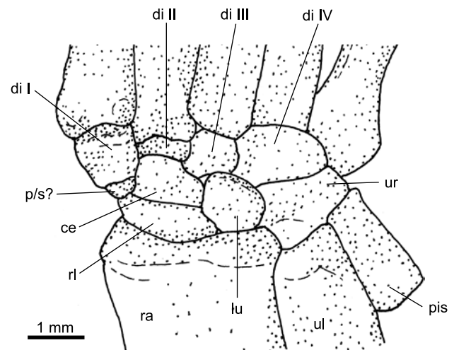
Fig. 12. Carpus of Zhangheotherium quinquecuspidens Hu, Wang, Luo, and Li, 1997, IVPP V7466, Jianshangou Valley, Liaoning Province, China, Barremian, right carpus, dorsal view. Abbreviations: di, distal carpal; ce, centrale; lu, lunate; p/s, prepollex/sesamoid, probably a fragment; pis, pisiform; ra, radius; rl, radiale; ul, ulna; ur, ulnare.
