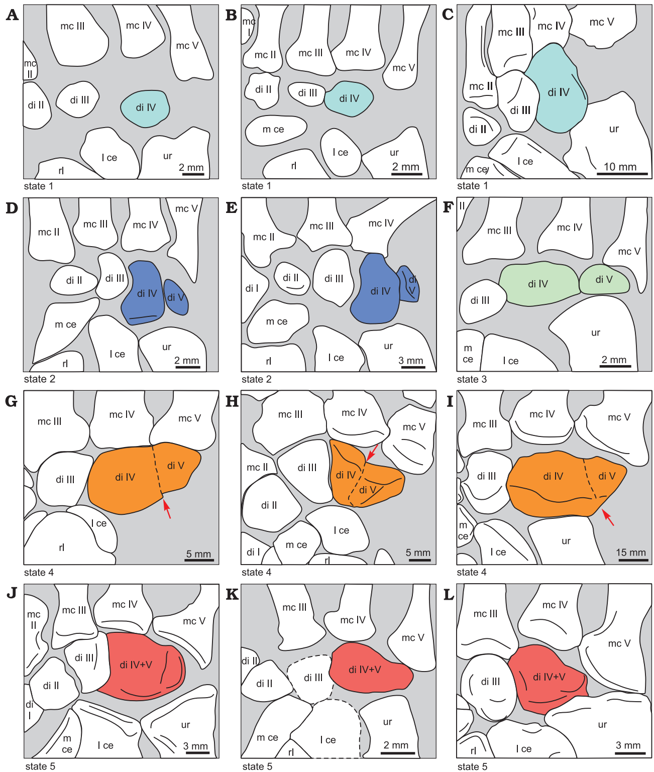
Fig. 16. Selected specimens showing the different states of distal carpal V in gorgonopsians, therocephalians, and cynodonts, all in dorsal view (except A, ventral view). A. Olivierosuchus parringtoni (Brink, 1965), BP/1/3973, left carpus. B. Tetracynodon darti Sigogneau, 1963, AM 3677, right carpus. C. Trucidocynodon riograndensis Oliveira, Soares, and Schultz, 2010, UFRGS PV-1051T, right carpus. D. Procynosuchus delaharpeae Broom, 1937, BP/1/591, right carpus. E. Procynosuchus delaharpeae Broom, 1937, NHMUK PV R 37054, right carpus. F. Ictidosuchoides longiceps Broom, 1920, CGS CM86-655, right carpus. G. Arctognathus curvimola (Owen, 1876), SAM-PK-3329, right carpus. H. Theriognathus microps Owen, 1876, NHMUK R 5694, right carpus. I. Gorgonopsian BP/1/1210, left carpus (reversed). J. Glanosuchus macrops Broom, 1904, SAM-PK-K7809, left carpus (reversed). K. Ictidosuchoides longiceps Broom, 1920, or Ictidosuchops intermedium (Broom, 1938), BP/1/2294, right carpus. L. Procynosuchus delaharpeae Broom, 1937, RC92, right carpus. Colours show the different states of distal carpal IV and V. Arrows show the stippled fusion lines between distal carpals IV and V. Abbreviations: mc, metacarpals; di, distal carpals; l ce, lateral centrale; m ce, medial centrale; rl, radiale; ur, ulnare.
