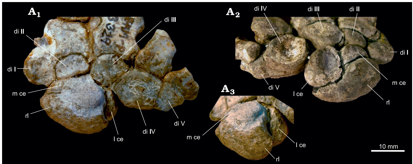
Fig. 11. Part of the carpus of Arctognathus curvimola (Owen, 1876), SAM-PK-3329, Oudeberg, Graaff-Reinet, South Africa, Cistecephalus Assemblage Zone, Lopingian. Dorsal (A 1 ), ventral (A 2 ), and dorsolateral (A 3 ) views, showing the fusion lines between the radiale and the centralia. Abbreviations: di, distal carpal; l ce, lateral centrale; m ce, medial centrale; rl, radiale.
