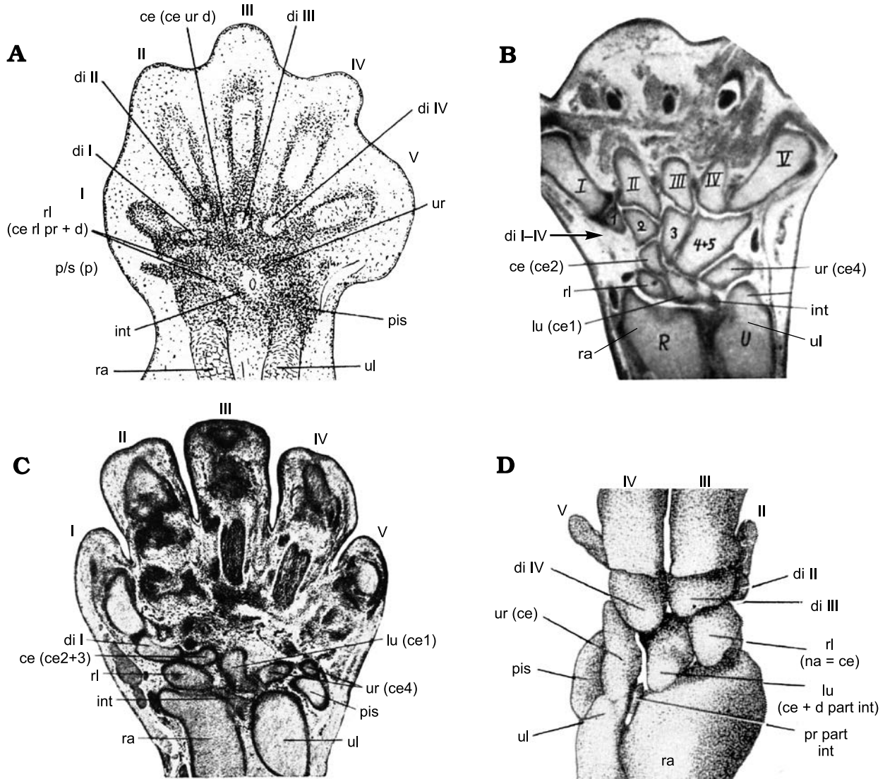
Fig. 14. Interpretation of the cartilaginous anlagen of the embryological carpus of different mammals by different authors. Whenever the radiale, ulnare or lunare have been interpreted previously as homologues of a centrale, the details are given in brackets following the abbreviations in the figures. A. Microcebus myoxinus Peters, 1852, 10.2 mm neck-rump length (from Schmidt-Ehrenberg 1942: 61, fig. 10, courtesy of Revue Suisse de Zoologie). B. Tarsius spectrumgurskyae Shekelle, Groves, Maryanto, and Mittermeier, 2017, 20.5 mm body length, (from Holmgren 1952: 80, fig. 93, reproduced with permission of Acta Zoologica, © The Royal Swedish Academy of Sciences, all rights reserved). C. Talpa europaea Linnaeus, 1758, 15 mm body length (from Kindahl 1942b: 270, fig. 4, courtesy of Sächsisches Staatsarchiv, Staatsarchiv Leipzig). D. Ovis aries Linnaeus, 1758, 38 mm body length, three-dimensional reconstruction of the left carpus in dorsal aspect (from Slabý 1967: pl. 6: 30). Abbreviations: ce, centrale; d, distal; di, distal carpal; int, intermedium; lu, lunare; na, naviculare; p, prepollex; p/s, prepollex/sesamoid; pis, pisiform; pr, proximal; ra, radius; rl, radiale; ul, ulna; ur, ulnare.
