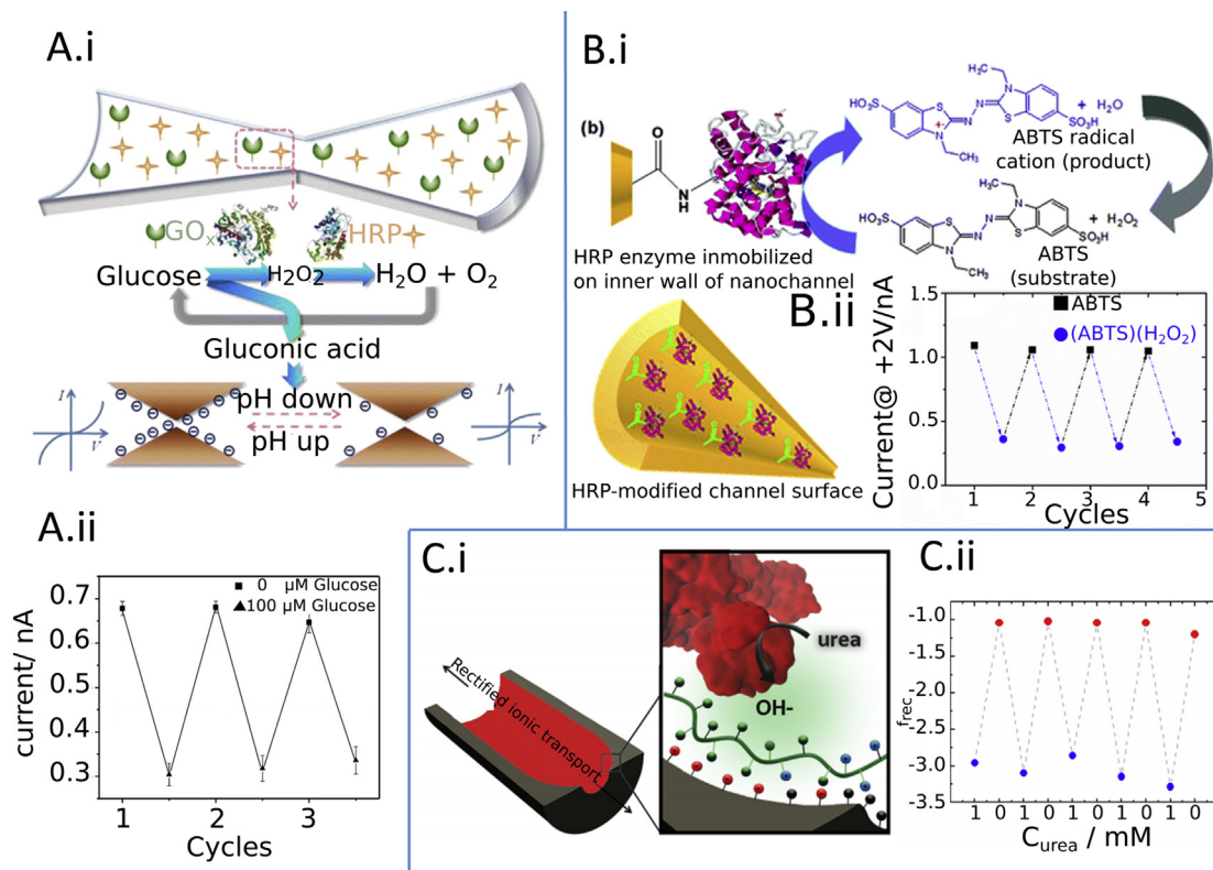
Fig. 2. Examples of signal amplification strategies for nanochannel sensing. A.i) An hourglass nanochannel is modified by glucose oxidase (GOx) and horseradish peroxidase (HRP). In the presence of glucose, the enzymatic reactions trigger a decrease of the pH within the channel, which protonates surface-bound carboxylate groups and, therefore, decreases the net surface charge of the channel and lowers its conductance (see effect of glucose on current in panel A.ii). Reproduced and adapted with permission from Ref. [11]. Copyright 2014 American Chemical Society. B.i) The inner surface of a conical nanochannel is modified by horseradish peroxidase. In the presence of \text{H}_2\text{O}_2 and ABTS, the channel conductance decreases because of the formation of \text{ABTS}^{\bullet+} (see effect of \text{H}_2\text{O}_2 on current in panel B.ii). Reproduced and adapted with permission from Ref. [76]. Copyright 2011 American Chemical Society. C.i) An asymmetrically shaped nanochannel is modified with a layer of PAH (a weak polyelectrolyte) and a second layer of urease. Hydrolysis of urea by urease increases the inner pH within the channel, which shifts the surface charge from positive to negative and, therefore, reverts the direction of current rectification (see effect of urea of current rectification ratio in panel C.ii). Reproduced and adapted with permission from Ref. [77]. Copyright 2018 American Chemical Society.
