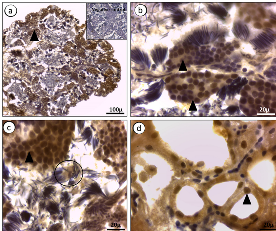
Figure 3. a) Expression of the PCNA cell proliferation protein in the transversal section of the testicle of S. acuminatus . b-c) Details of the PCNA positive spermatogenic cells line (circle). d) Expression of the PCNA cell proliferation protein in a cross section of the kidney of S. acuminatus . References: Arrow: PCNA positive cells.
