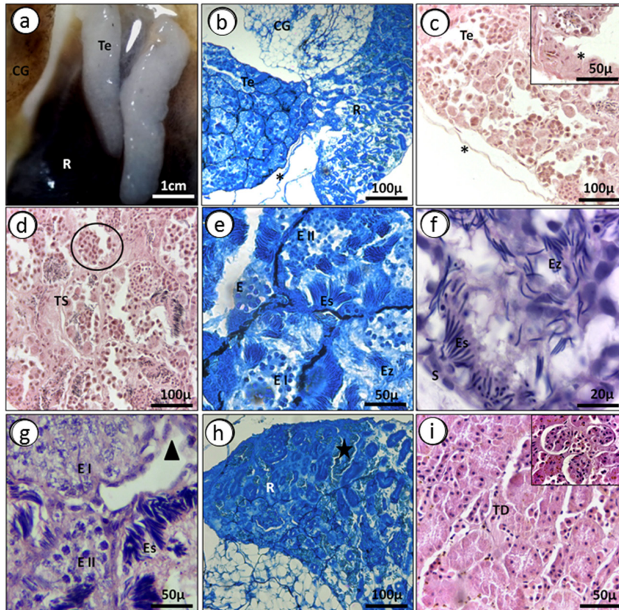
Figure 2. a) Detail of the testes with tunica albuginea without pigmentation, kidneys and fat bodies in S. acuminatus . b) Sagittal section of testicles, kidneys and fat body (Staining: Coomassie blue). c) Transversal section of the testicle with detail of the tunica albuginea (Staining: H-E). d) Detail of the seminiferous tubules with cysts (Staining: H-E). e) Detail of the cell types each spermatogenic cyst and seminiferous tubules surrounded by melanocytes (Staining: Coomassie blue). f) Detail of plume of spermatids attached to the Sertoli cell (Staining: PAS). g) Detail of the interstitial cells and Leydig cells (Staining: H-E). h) Transversal section of the kidney, with emphasis on the convoluted tubules that are part of the sexual segment (Staining: Coomassie blue). i) Detail of the convoluted tubules of the hypertrophied sexual segment with positive PAS cells and detail of the genital glomerulus (Staining: PAS). References: Te: testicle. CG: fat bodies. R: kidney. Asterisk: tunica albuginea. TS: seminiferous tubule. Circle: cistos. Me: melanocytes. E: spermatogonia. El: primary spermatocytes. Ell: secondary spermatocytes. Esp: spermatids. Ez: sperm. S: Sertoli cells. Star: hypertrophied contiguous tubules. TD: distal contiguous tubules. Arrowhead: Leydig cell.
