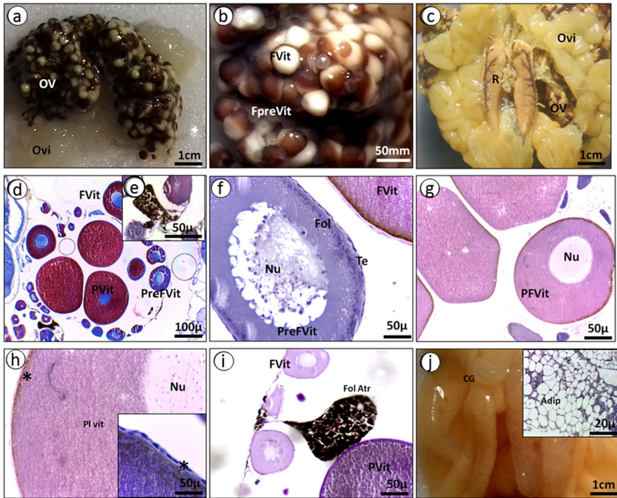
Figure 1. a) Detail of the ovary and oviduct of S. acuminatus . b) Detail of the cell types present in the ovary. c) Relationship between the position of the kidneys and the ovary and its vascularization. d) Transversal section of the ovary at the reproductive stage (Staining: Masson's Trichrome). e) Detail of a pre-vitellogenic follicle (Staining: PAS). f) Atretic pre-vitellogenic follicle. g) Detail of a vitellogenic follicle (H-E Staining). h) Detail of an atretic vitellogenic follicle (Staining: H-E). i) Fat bodies and detail in histological section (Staining: H-E). References: arrow: revetment epithelium. Ov: ovary. Ovi: oviduct. R: kidney. Fvit: vitellogenic follicle. FpreVit: Pre-vitellogenic follicle. Pvit: post-vitellogenic. Fol Atr: atretic follicle. Pl vit: viteline platelets. Nu: nucleus. Fol: follicular cells (*). Te: tecal cells, CG: fat body. Adip: adipocytes. Mes: mesovarium.
