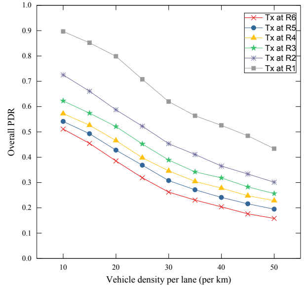
Fig. 8: Overall packet delivery ratio (PDR) at an intersection.
