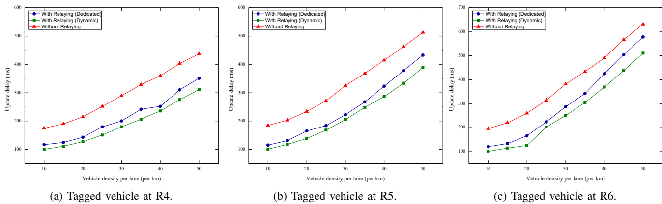
Fig. 14: Communication latency comparison.
