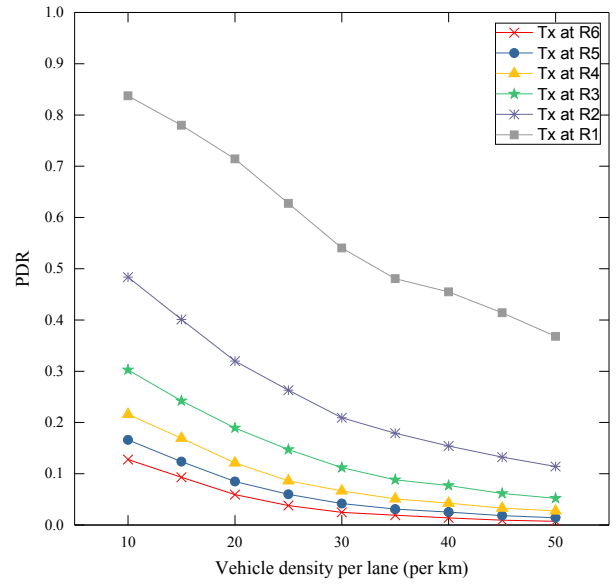
Fig. 7: Packet delivery ratio (PDR) at perpendicular street.
