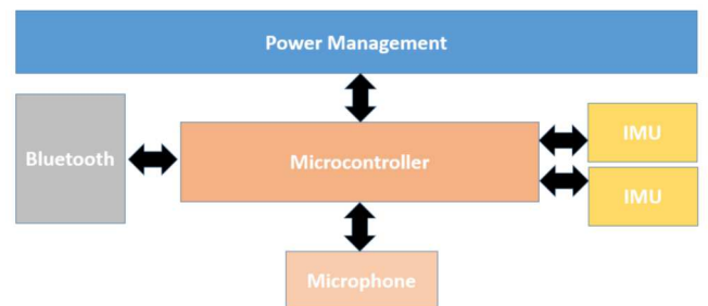
Fig. 2. System architecture for the bruxism diagnostic system
