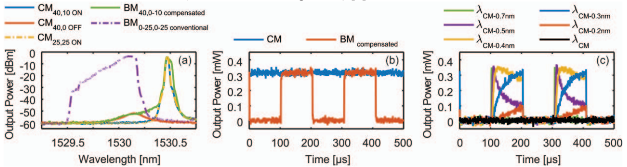
Fig. 2. (a) CM and BM spectra (CW, max/hold, 500 scans, resolution: 20pm, sensitivity: -55dBm); (b) Output power after 0.22nm OBF for the proposed approach and (c) for the conventional BM approach with various OBF tuning values with respect to \lambda_{CM} .
