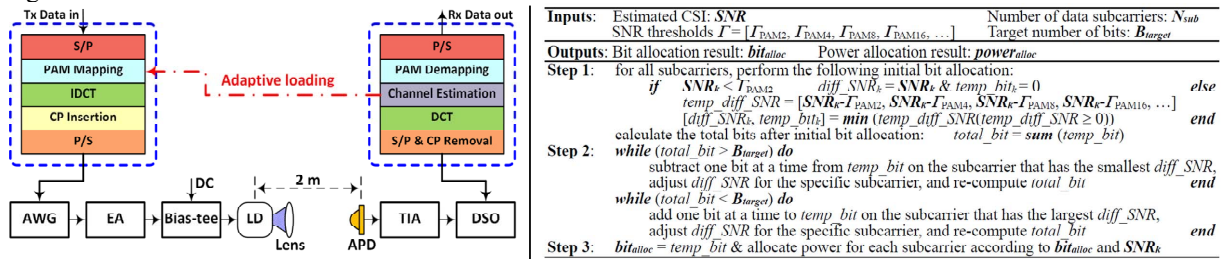
Fig. 1. Experimental setup and the corresponding DSP blocks of the OWC system (left), and the pseudo code of the proposed SNR-threshold based adaptive bit and power loading algorithm for PAM-fast-OFDM (right).
