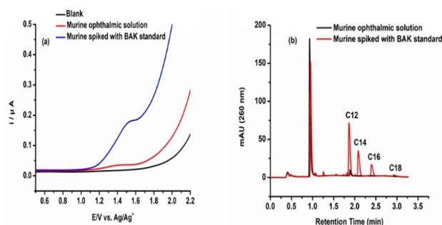
Fig. 6. (a) SWVs of Murine ophthalmic solution and spiked with 40 µg/mL of BAK on the bare BDD electrode vs. Ag/Ag + in 10 mM TBAH/ACN. (b) HPLC-UV gradient analysis of Murine ophthalmic solution and spiked with 3 mg/mL of BAK analyzed by gradient HPLC-UV. Mobile phase: A: 0.05 % TFA in H 2 O, B: 0.05 % TFA in (ACN: IPA; 50:50), flow rate: 0.3 mL/min, temperature 30 °C.
