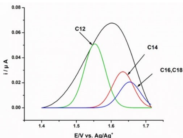
Fig. 4. Resolved SWV of the standard mixture at 80 µg/mL of BAK after the application of peak deconvolution using Origin Pro 8.5.1. on the BDD electrode vs. Ag/Ag + using 10 mM TBAH/ACN.
