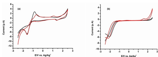
Fig. 1. CV response in the absence (black) and presence (red) of 80 µg/mL for BAK on the (a) GC and (b) BDD electrodes vs. Ag/Ag + . Electrolyte: 10 mM TBAH/ACN with a scan rate 100 mV/s.
