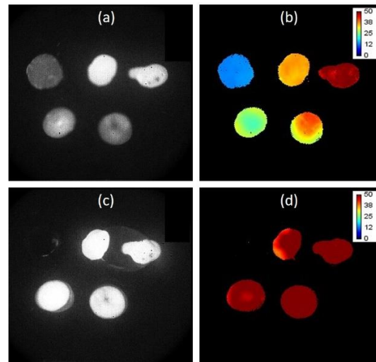
Figure 2. Images of the polymer based phosphorescent coating spotted on polyester film (spot size \sim 2\text{-}3 \text{ mm} ): in the oxygenated state in (a) intensity and (b) lifetime( \mu\text{s} ) scale; in the de-oxygenated state in (c) intensity and (d) PLIM ( \mu\text{s} ) mode, 22^\circ\text{C} .
