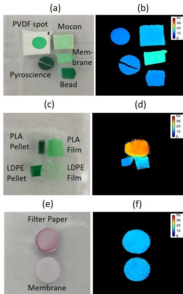
Figure 4. Sets of commercial and custom-made O 2 sensors imaged with the Tpx3Cam imager. (a) Photograph and (b) PLIM image of the PtBP based sensors in various forms; (c) Photograph and (d) PLIM image of LDPE-PLA based PtBP sensors and (e) Photograph and (f) PLIM image of the two PtOEPK based sensors.
