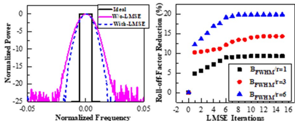
Figure 1: Example LMSE spectral shaping. (left) comparison of ideal filter shape (rectangle), shaping after WSS (solid line), and after LMSE algorithm (dashed line). (right) Roll-off factor improvement for each iteration, for a number of filter widths.
