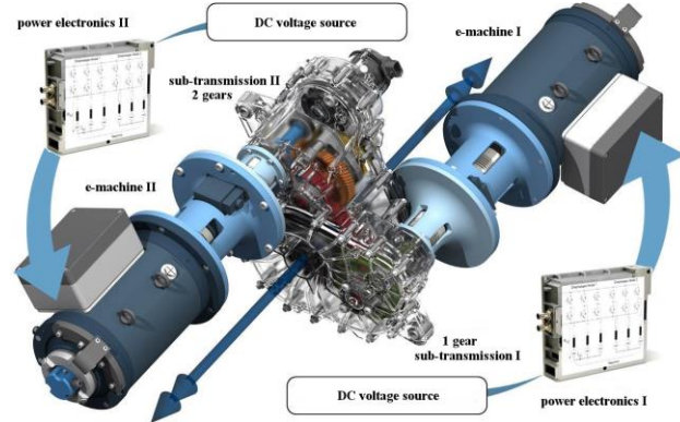
Figure 2: Drivetrain of the Speed2E Project, covering speed of up to 30,000 rpm for two sub transmissions [21]
