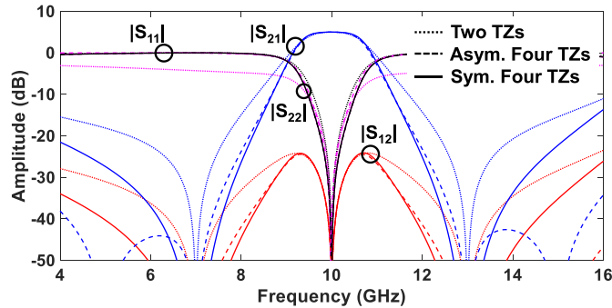
Fig. 9. Comparison of the S-parameters of the NBPFs in Fig. 6 (dotted lines) and Fig. 8 (solid and dashed lines).
