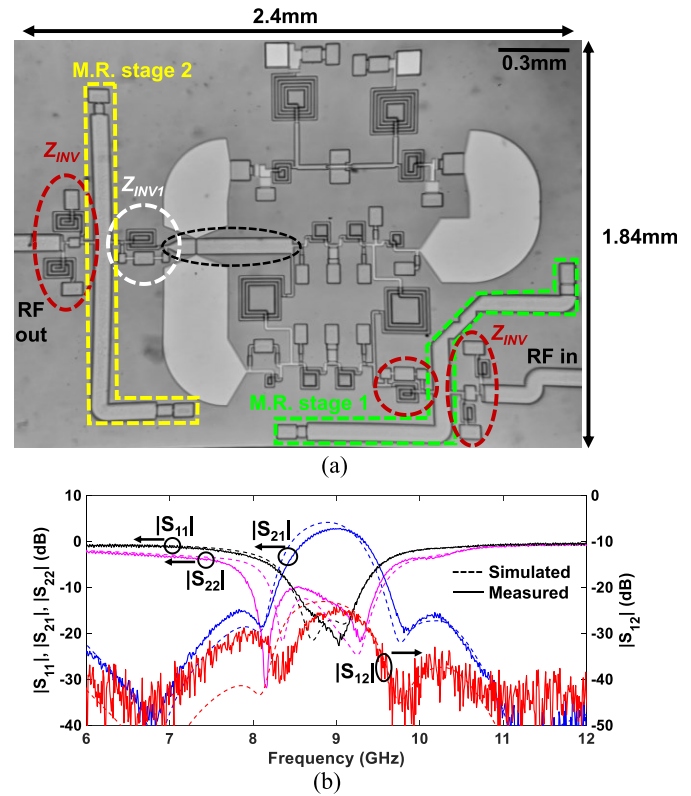
Fig. 14. (a) Photograph for the manufactured three-resonator/four-TZ prototype based on the block diagram in Fig. 8(a). The second multi-resonant stage is circled in yellow, Z_{INV} is circled in red, Z_{INV1} is circled in white, the line needed to prevent overlap between the NFS is circled in black, and the multi-resonant stage 1 is circled in green. (b) Measured and EM-simulated S-parameters for the three-resonator/four-TZ prototype in (a).
