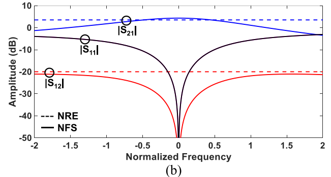
Fig. 2. NFS with enhanced power transmission response in the forward direction ( |S_{21}| ) and complete RF signal cancellation in the reverse one ( |S_{12}| ). (a) Block diagram and symbol, white and grey rectangles represent 90^\circ -long transmission lines at f_{cen} , white triangle: NRE with or without gain. (b) Ideal power transmission ( |S_{21}| ), isolation ( |S_{12}| ), and reflection ( |S_{11}| , |S_{22}| ) responses of the NFS (solid lines) and its corresponding NRE (dashed lines). The element values for this example are: Z_A = 11.9 \Omega , Z_B = 71.1 \Omega , Z_C = 12.1 \Omega , NRE S-parameters: S_{11} = 0 , S_{12} = 0.17 , S_{21} = 1.5 , and S_{22} = 0 .
