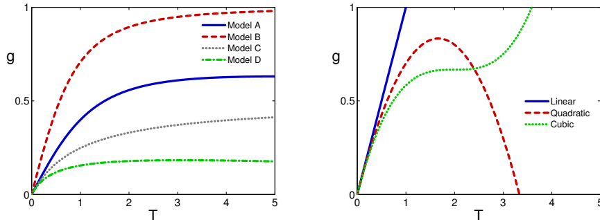
FIGURE 3. Left. Model A: g(T) = \beta T + \alpha \left(1 + \frac{\gamma}{2} T^2\right)^n T ; Model B: g(T) = \frac{T}{(1+|T|^r)^{1/r}} ; Model C: g(T) = \alpha \left\{ \left[1 - \exp\left(-\frac{\beta T}{1+\delta|T|}\right)\right] + \frac{\gamma T}{1+|T|} \right\} ; Model D: g(T) = \alpha \left(1 - \frac{1}{1+\frac{T}{1+\delta|T|}}\right) + \beta \left(1 + \frac{1}{1+\gamma T^2}\right)^n T , where \alpha, \beta, \gamma, \delta, n and r > 0 are constants. Right. General linear, quadratic and cubic nonlinearities.
