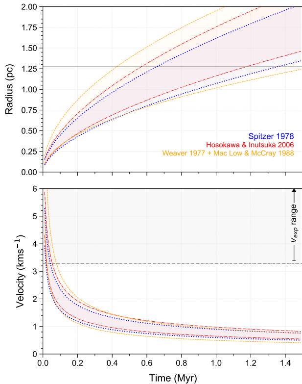
Figure 6. The top panel shows analytic predictions for the time evolution of the radii of expanding H II regions from various models (see text for details). The blue dotted curve indicates expansion driven by the thermal pressure of photoionised gas Spitzer (1978) . The red dot-dashed curve is the same but with a slight modification from Hosokawa & Inutsuka (2006) . The orange dashed curves describe the radial expansion driven by stellar winds for stars of different spectral types consistent with our measurement of N_{\text{LyC}} ( Weaver et al. 1977 ; Mac Low & McCray 1988 ). The horizontal black line represents the radius of the arc R_{\text{arc}} = 1.3 pc. The bottom panels show the corresponding time evolution of the expansion velocity. The black shaded region indicates the range of expansion velocity derived from the different methods presented in § 3.2 (note that this has been truncated for clarity, as indicated by the black arrow). The horizontal dot-dashed line reflects the lower limit of the expansion velocity estimates shown in Figure 4.
