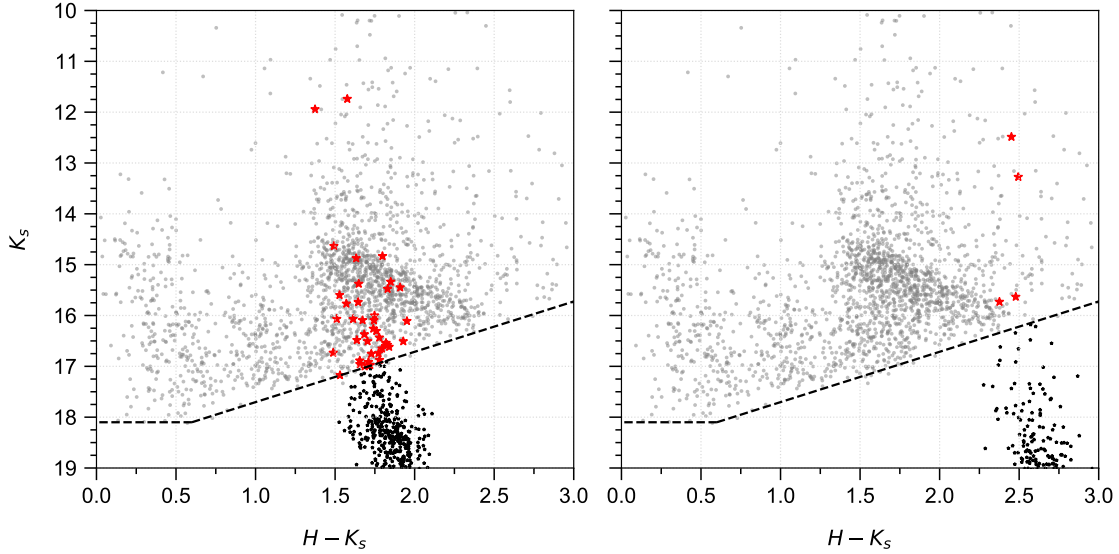
Figure 7. Colour-magnitude diagram K_s versus H - K_s corresponding to the region containing G0.253+0.016 (see Fig. 2 in Nogueras-Lara et al. 2021a). Grey dots represent real stars from the GNS survey (Nogueras-Lara et al. 2018, 2019). The red and black stars correspond to the synthetic stellar population of a young (0.5 Myr) cluster of mass 500 M_\odot . The red and black stars detections and non-detections from the synthetic population, respectively, considering the detection limit of the data (black dashed line). The left and right panels assume an extinction of A_{K_s} = 2 and 3 mag, respectively, with the latter indicating fewer detections of cluster members.
