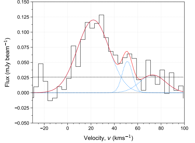
Figure 5. Radio recombination line spectrum extracted from within the circle presented in Figure 3. This spectrum was created by stacking a total of seven radio recombination lines, namely H114 \alpha , H113 \alpha , H110 \alpha , H109 \alpha , H101 \alpha , H100 \alpha , and H99 \alpha . The horizontal dotted line indicates the 0.0 line and the horizontal dashed line indicates 3.0 \times \sigma_{\text{rms}} ( 0.026 \text{ mJy beam}^{-1} ). The red curve indicates a three component Gaussian fit to the data. The component at lower velocities has a centroid velocity of 22.0 \pm 1.4 , closely matching the velocity of the molecular component of arc (Figure 2).
