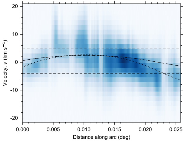
Figure 4. A position-velocity diagram extracted along the dotted ellipse presented in Figure 3. The 0.0 location is taken to be the lowest Galactic longitude point on the arc. The colour scale reflects the peak amplitude of the HNC emission. The lines represent different models for the kinematics of the arc velocity field presented in the right panel of Figure 3. The horizontal dashed lines represent the most simplistic approach to estimating the expansion velocity, and reflect the half-width at half-maximum of the gradient-subtracted velocity distribution (see text for details), v_{\text{exp}} = 4.2 km s ^{-1} . The dot-dashed and dotted lines correspond to the model velocity fields described in § 3.2. The former of these models has a constant expansion velocity of v_{\text{exp}} = 3.3 km s ^{-1} . The latter also has constant expansion velocity, this time v_{\text{exp}} = 7.9 km s ^{-1} , but the model also includes a constant line-of-sight velocity of v_{0,\text{arc}} = -3.1 km s ^{-1} .
