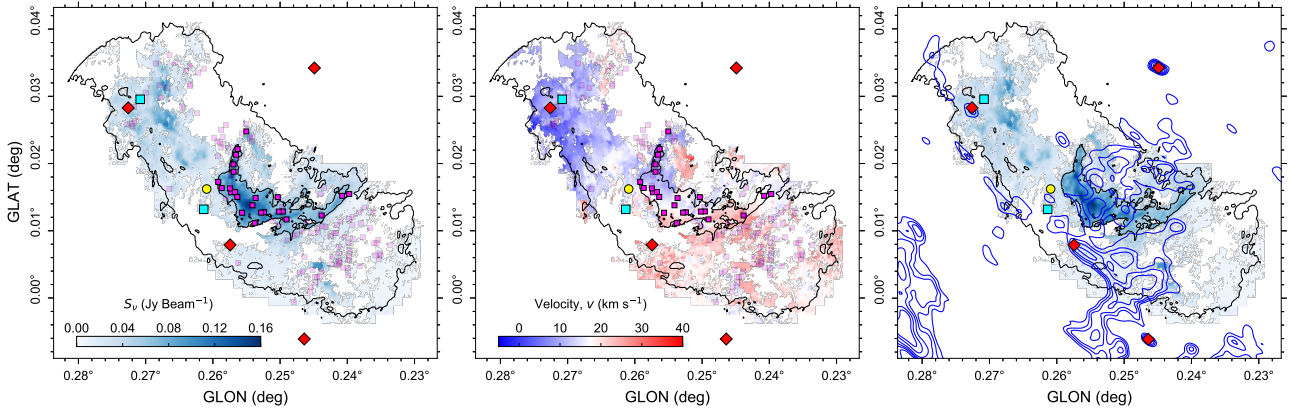
Figure 1. Left: The peak flux distribution associated with the arc’s parent sub-cloud identified in Paper 1. The colour scale shows the peak amplitude of all Gaussian components associated with the arc’s parent sub-cloud (derived from the fitting of the HNC data). The thick black contour highlights the arc itself. The thin black contour shows the boundary of G0.253+0.016 estimated from the integrated emission of HNC. We overlay the location of the H 2 O maser identified by Lis et al. (1994) as a yellow circle and the additional H 2 O masers identified by Lu et al. (2019a) as cyan squares. H II region candidates from Rodríguez & Zapata (2013) are shown as red diamonds. Purple squares indicate the locations of class I CH 3 OH masers and maser candidates identified by Mills et al. (2015). Transparent squares are those which lie outside of a \pm 6 \text{ km s}^{-1} velocity range around a 2-D velocity plane fitted to the ACORNs data (see text). Centre: The corresponding centroid velocity map of the arc’s parent sub-cloud. The symbols are equivalent to those in the left panel. Right: The peak flux distribution with the VLA radio continuum data overlaid as blue contours. Contours start at 3\sigma ( \sigma = 0.15 \text{ mJy beam}^{-1} ), then 5, 7, 10, 15, and 20\sigma (Butterfield et al. in preparation).
