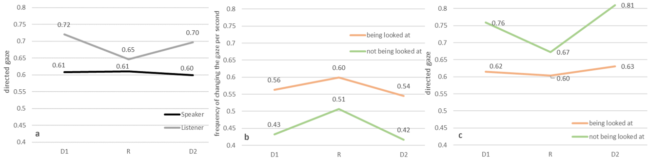
Figure 2: a: DG percent while being a speaker or a listener during each task. b: Gaze change frequency while being or while not being looked at during each task. c: DG percent while being or while not being looked at by task. The tasks are in chronological order (D stands for discussion (1 and 2) and R for recipe)
