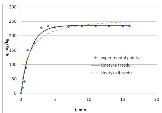
Fig. 8. The kinetics of the release of chlorides from the salt debris of grain size 0-20 mm to solution, T = 15°C, C 0 (saturated solution) = 187.15 mg / dm 3 .
