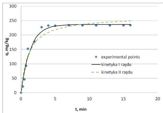
Fig. 7. The kinetics of the release of chlorides from the salt debris of grain size 0-10 mm to solution, T = 15°C, C 0 (saturated solution) = 187.15 mg / dm 3 .
