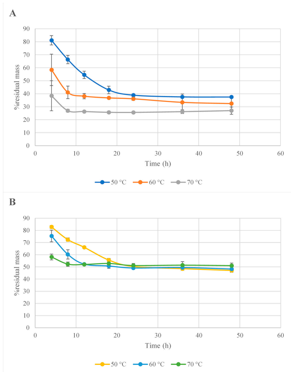
Figure 1. Residual mass percentage versus drying time for temperatures of 50, 60, and 70 °C in B. vulgaris (A) and C. monogyna (B).
