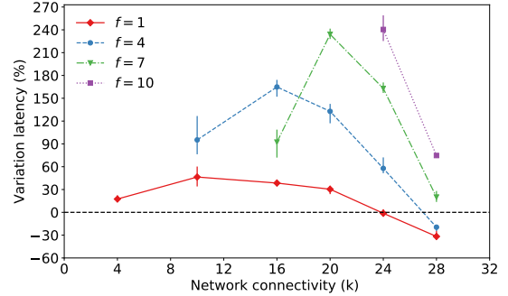
Fig. 5. MBD.11’s latency impact - N = 31 , 16KB payload.
