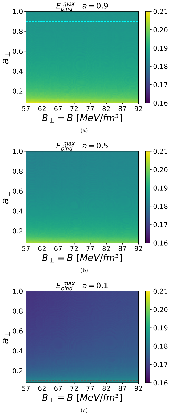
Figure 6. Binding energy profile for the full set of solutions of the perpendicular component of the interacting parameter and the bag parameter.
