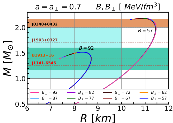
Figure 1. Mass-radius relation for anisotropic quark stars with a = a_{\perp} = 0.7 .
