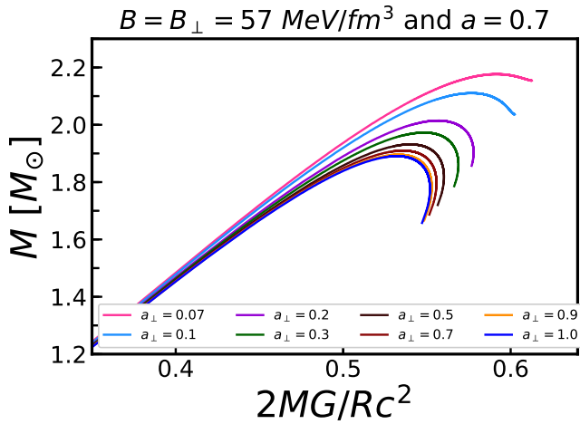
Figure 5. Compactness C of anisotropic QS with B = 57 .
