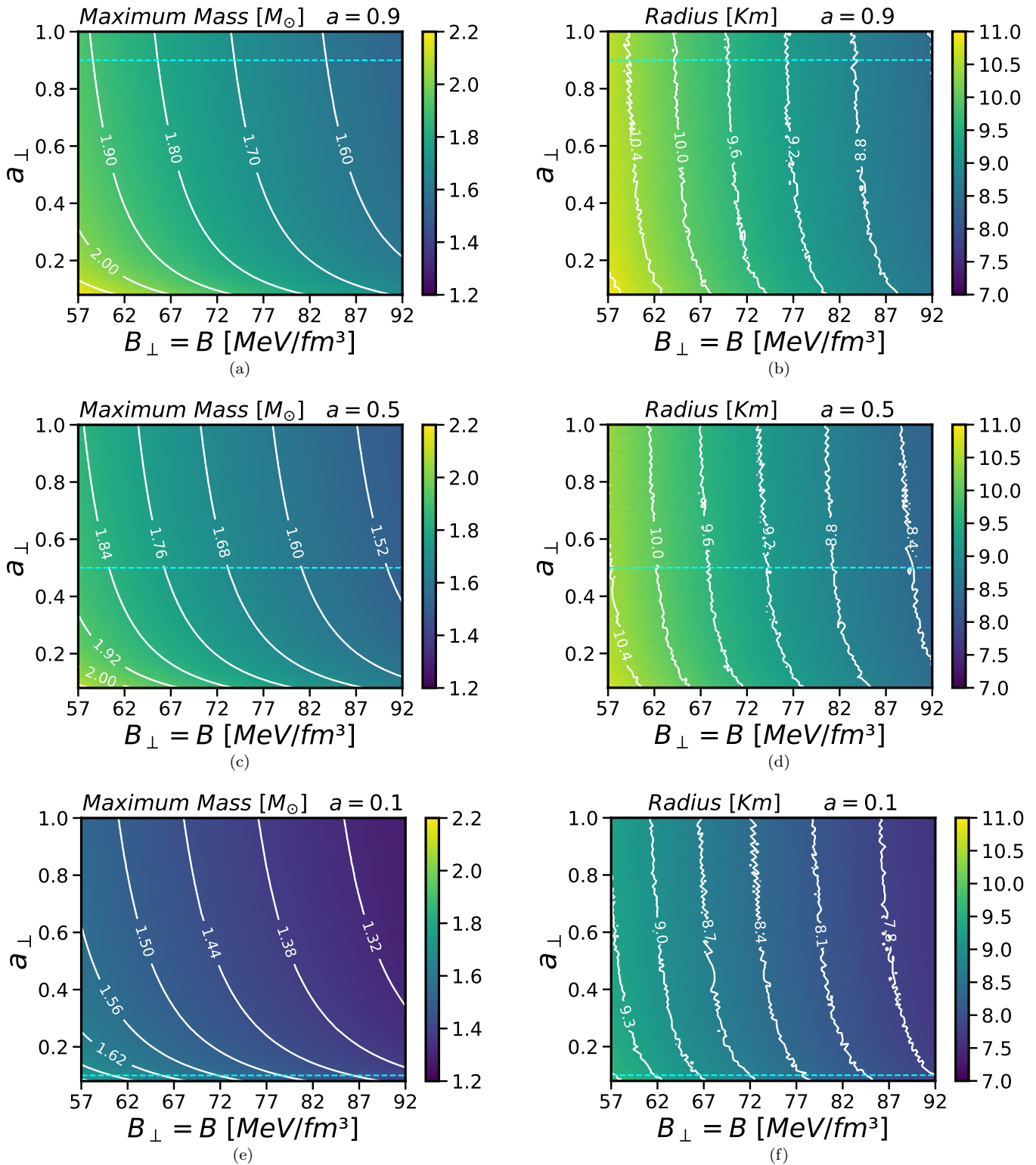
Figure 4. Maximum masses and their corresponding radii for the full range of values of a_{\perp} and B_{\perp} . The white lines are all QS in which the maximum mass and radius has the same value, and the cyan colored lines are the isotropic cases ( a = a_{\perp} ).
