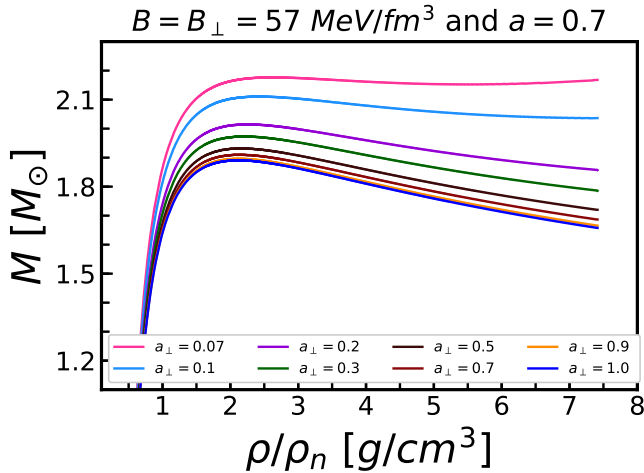
Figure 3. Mass-density relation for anisotropic quark star in where \rho_n = 2.4 \times 10^{14} \text{ g/cm}^3 .
