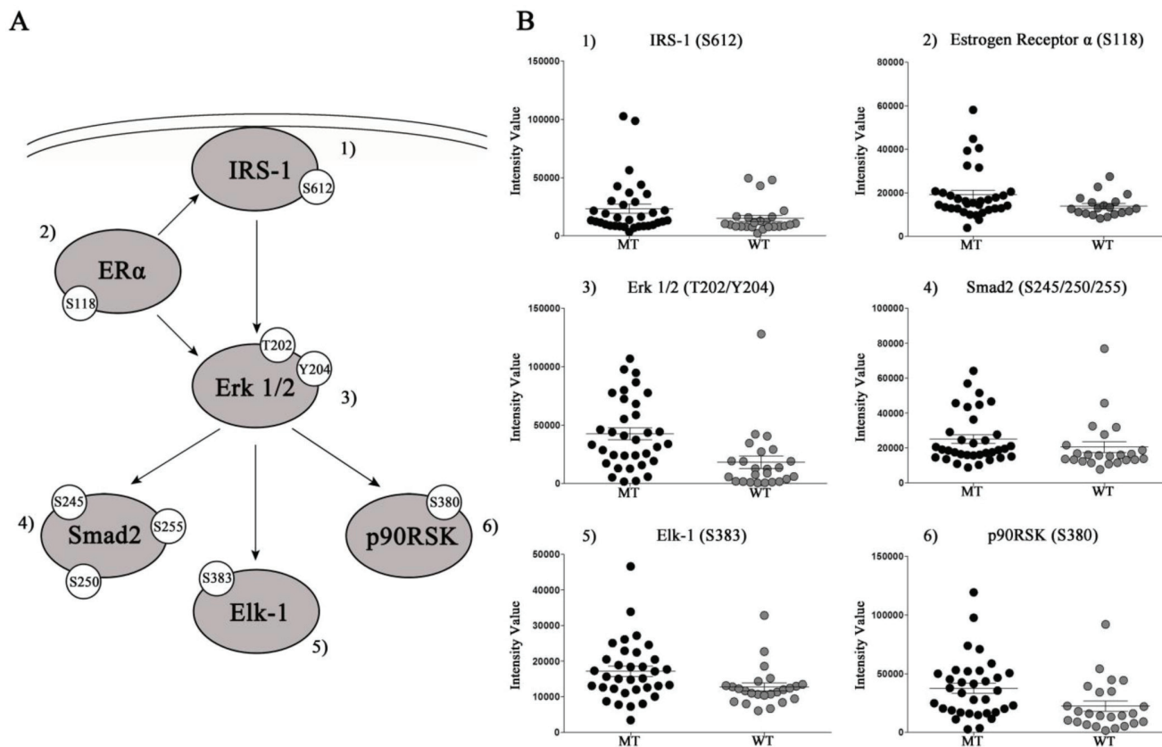
Figure 2: Panel A: Representation of selected proteins that were significantly higher in KRAS MT tumors. Panel B: Scatter plots of RPPA intensity values with mean and standard error of mean.
