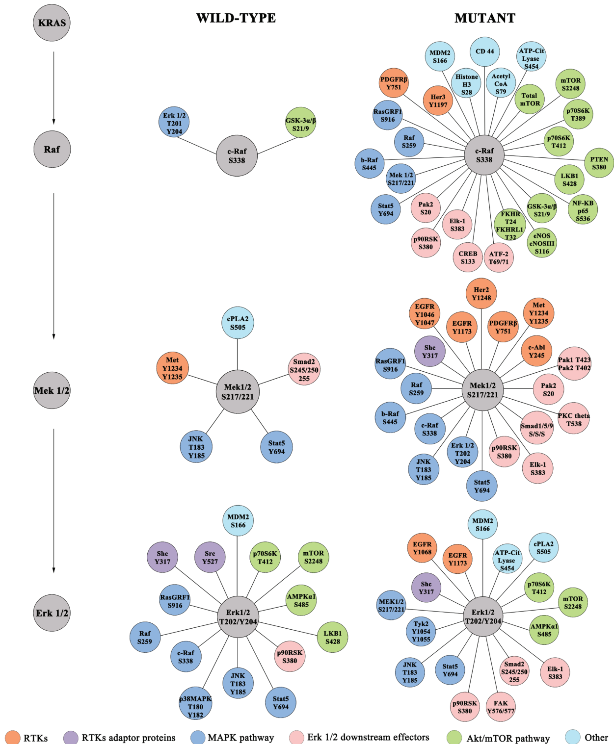
Figure 1: Correlation analysis of KRAS downstream substrates (activated c-Raf, Mek 1/2 and ERK 1/2) and expression/activation levels of 145 endpoints analyzed. Only correlations with p < 0.0003 are shown.
