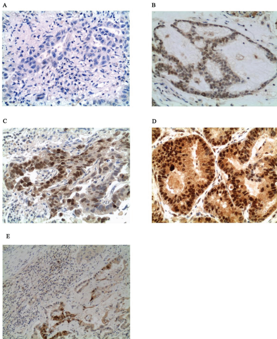
Figure 3: Example of ER- \alpha S118 staining by IHC (x400 magnification). Panel A, B, C, and D show no activation, weak activation (1+), moderate activation (2+), and strong activation (3+) respectively. Panel E shows activation of ER- \alpha S118 in the adenocarcinoma component of the sample with mixed adeno-squamous histology.
