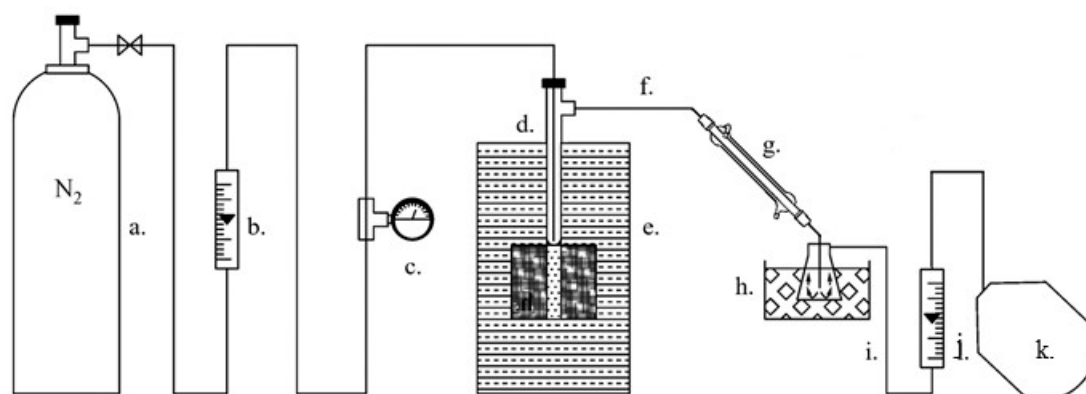
Figure 4. Pyrolysis experimental set-up: (a) N 2 cylinder, (b) upstream flowmeter, (c) manometer, (d) quartz tube reactor, (e) electric furnace, (f) glass tube connector, (g) glass water condenser, (h) ice-bath cooled conical flask, (i) connection tygon tube, (j) downstream flowmeter, (k) gas sample bag.
